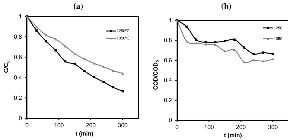
Figure 8. (a) Degradation of Norfloxacin and (b) COD removal vs time for two different ceramic electrodes (sintered at 1050 and 1250 °C) at an applied potential of 2.5 V.
