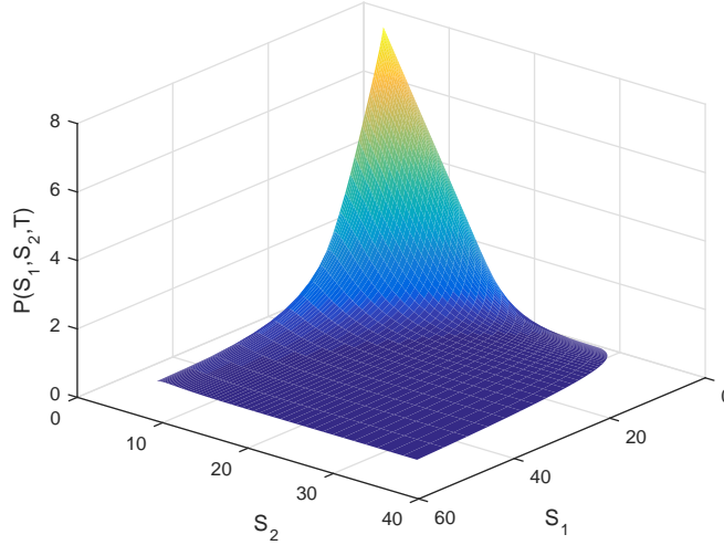
Figure 4: Reliable basket option price of Example 2 at \tau = T for h = 0.2 .
