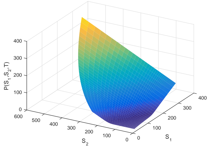
Figure 8: Basket call option price with parameters (50) at \tau = T .
