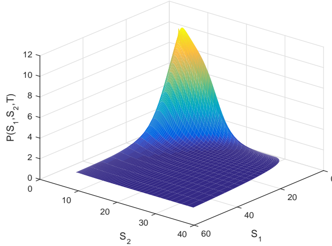
Figure 6: Wrong basket option price of Example 2 at \tau = T with broken stability conditions ( k = 0.1 , h = 0.2 ).
