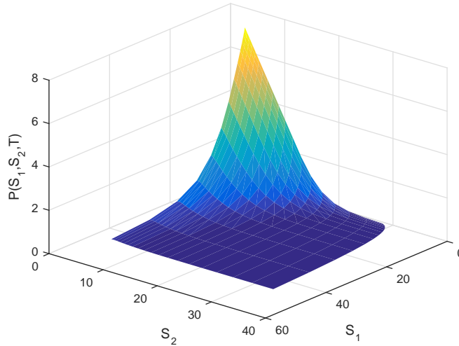
Figure 3: Reliable basket option price of Example 2 at \tau = T for h = 0.5 .
