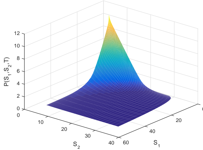
Figure 5: Wrong basket option price of Example 2 at \tau = T with broken stability conditions ( k = 0.05 , h = 0.2 ).
