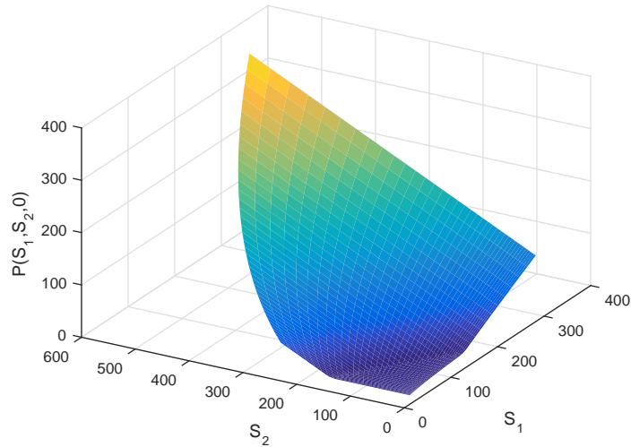
Figure 9: Basket call option price with parameters (50) at \tau = 0 .
