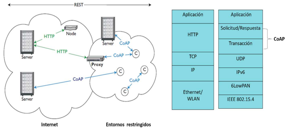
Figura 2.17: Funcionalidad de CoAP y HTTP (Adaptado de (Bormann et al. , 2012))
