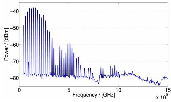
Fig.4. Measured spectrum of the monocycle at base-band after fiber transmission.
