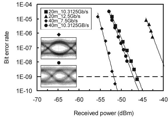
Fig. 31. Measured BER levels for multi-gigabit data transmission after 20 and 40m wireless path length.
