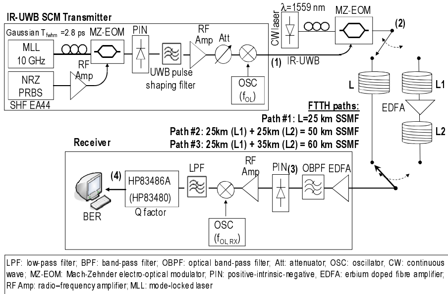
Fig.1. IR-UWB transmission in FTTH demonstration set-up.
