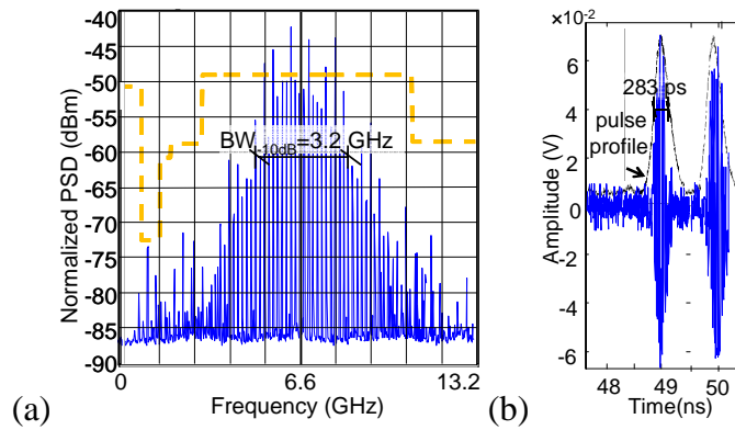
Fig.2. IR-UWB (a) RF spectrum,(b)Electrical signal and pulse profile
