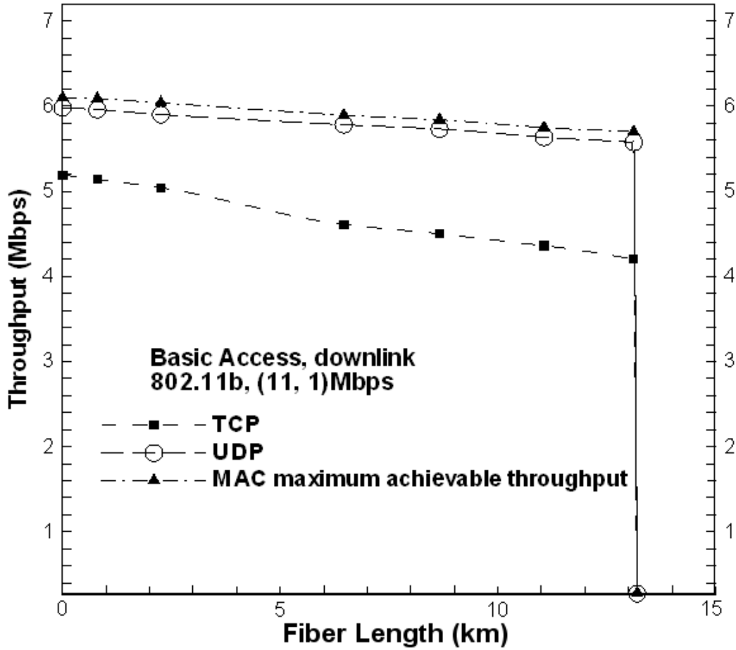
Fig.27. UDP, TCP and the MAC maximum achievable throughput -simulation results.
