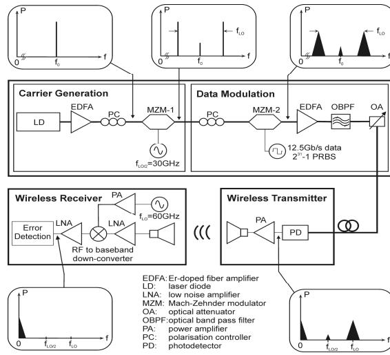
Fig. 29. Schematic of the 60GHz radio-over-fiber setup.
