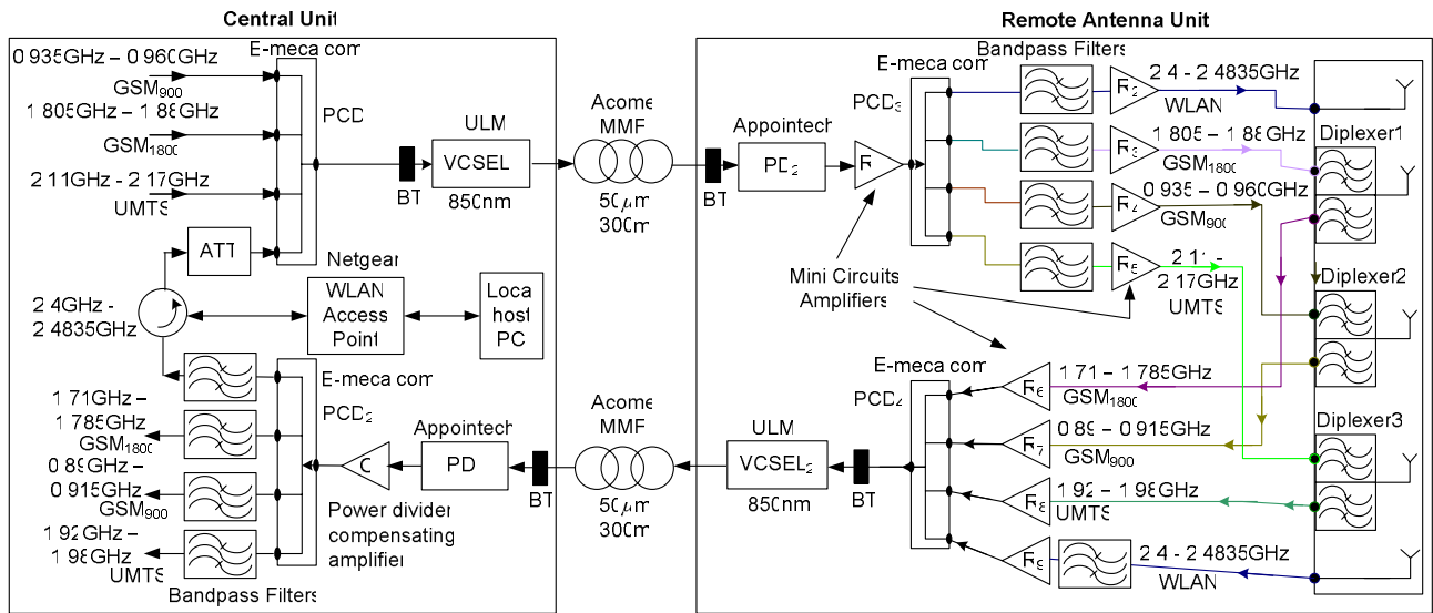
Fig. 16. Experimental set-up for multi-system transport over VCSEL-multimode fiber link [13].
