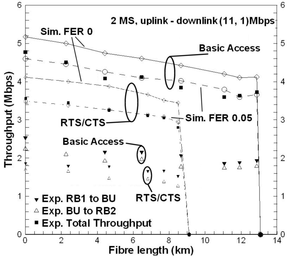
Fig.26. Variation of throughput with fiber length for TCP transmission (control data rate 1Mbps)
