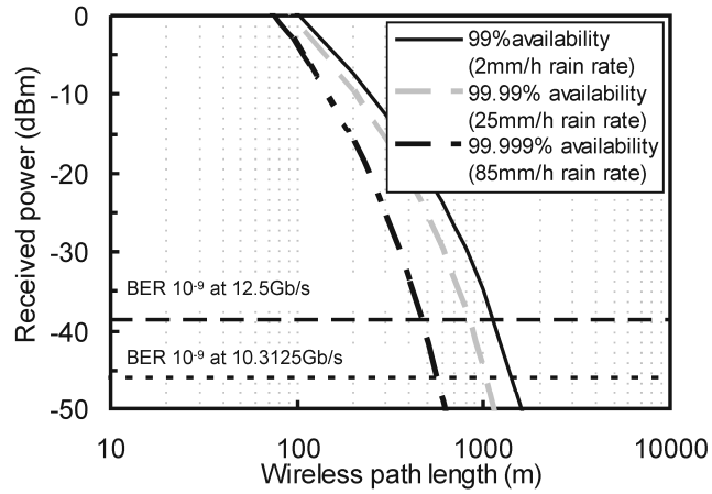
Fig. 32. Maximum wireless path lengths for different weather conditions.
