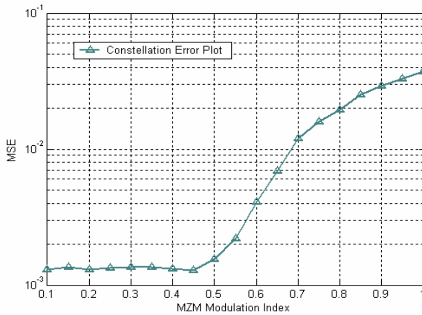
Fig.20. Constellation error at nominal MZM bias point.
