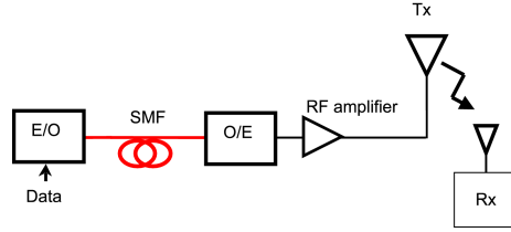
Fig. 9. A typical implementation of a radio over fiber system.
