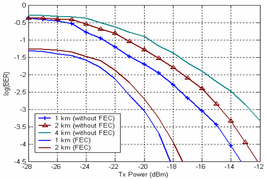
Fig.22. BER dependence on fiber length.
