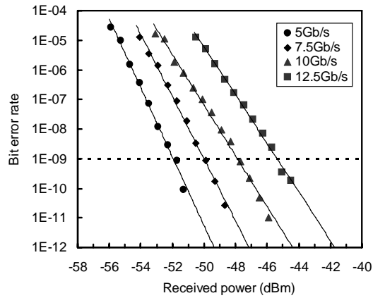
Fig. 30. BERs and 10Gb/s eye diagram after 2.5m wireless transmission.
