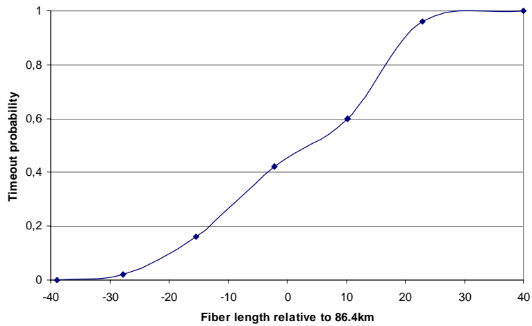
Fig. 28 Timeout uncertainty due to clock jitter.
