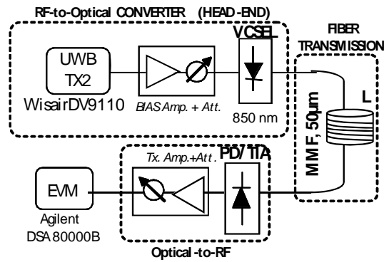
Fig. 7. Experimental setup for performance analysis of MB-OFDM UWB-on-fiber.
