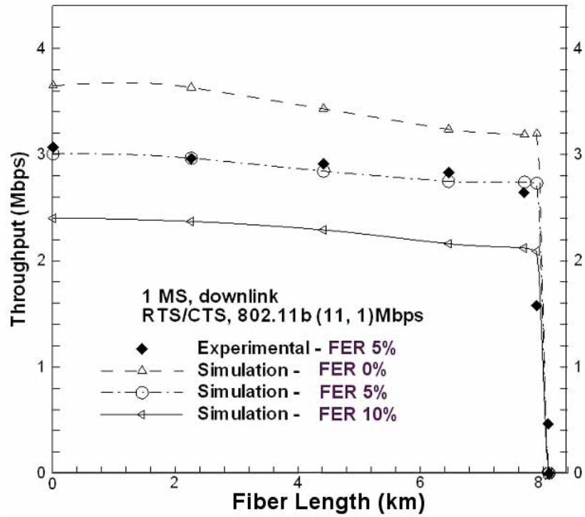
Fig.25. Variation of throughput with fiber length using RTS/CTS
