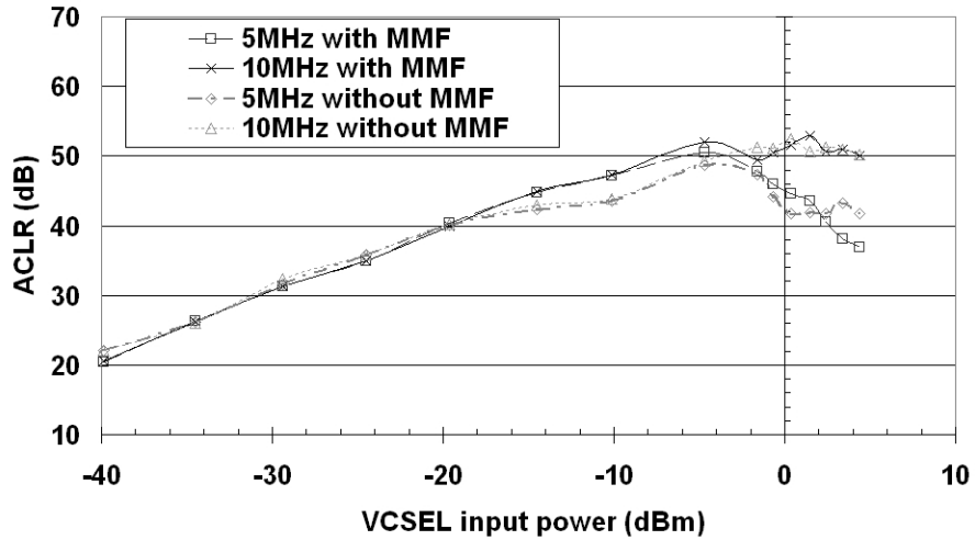
Fig.18 ACLR measurement for UMTS for the setup of Fig. 16, with all other systems present. The rising part of the curves is within conformance (although they are below the 50 dB and 45 dB requirements) as noise rather than signal leakage is measured in this region. [13].
