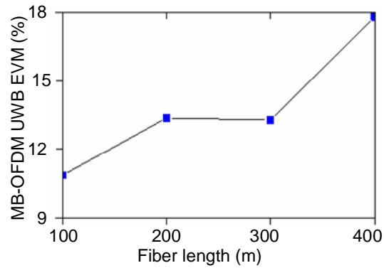
Fig.8 MB-OFDM UWB EVM results for different MMF lengths.
