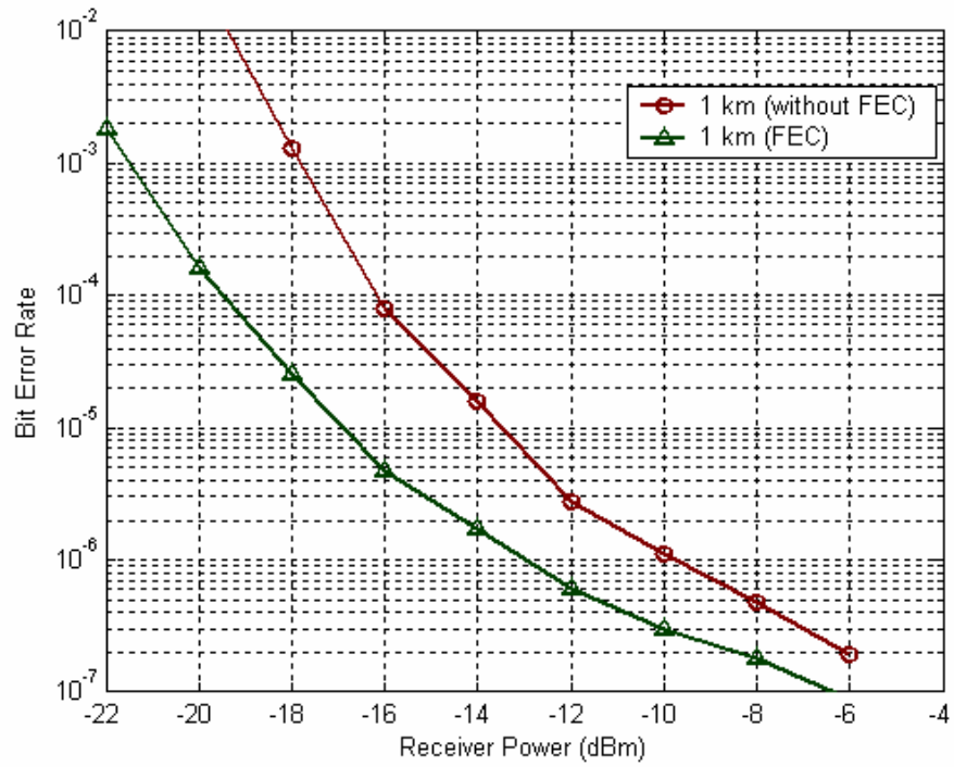
Fig.23. Receiver performance with FEC.
