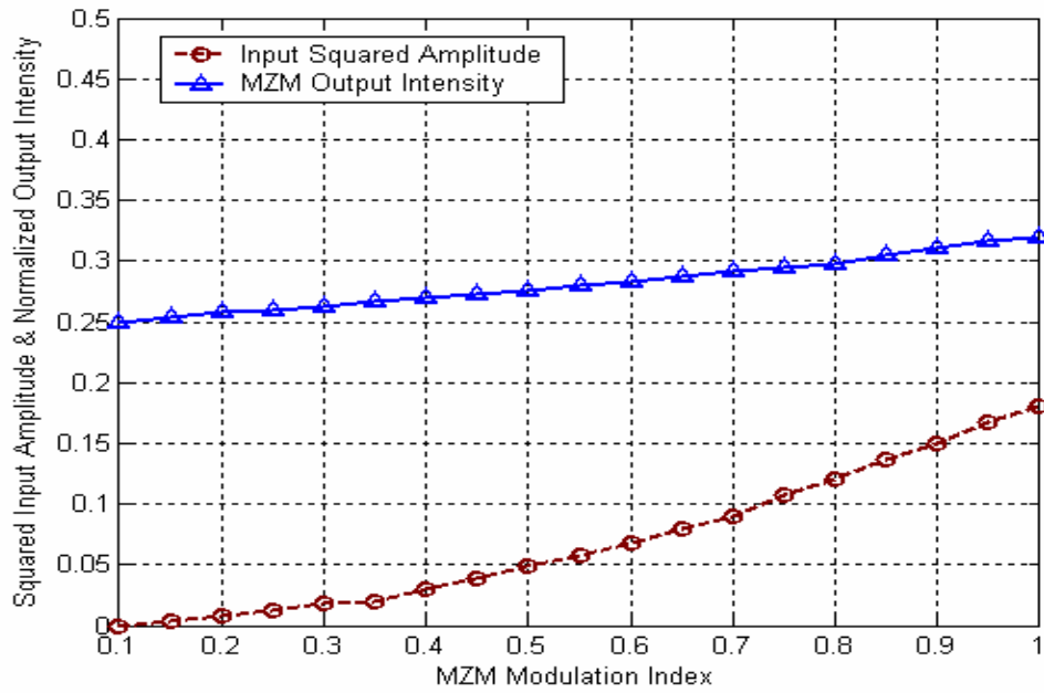
Fig.21. Signal amplitude & output intensity (nominal bias point).
