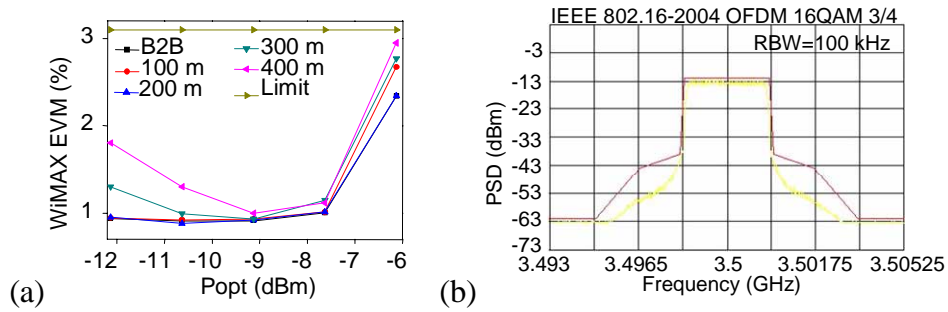
Fig.15. (a) WiMAX EVM measurements results and (b) measured conformance with spectral mask.
