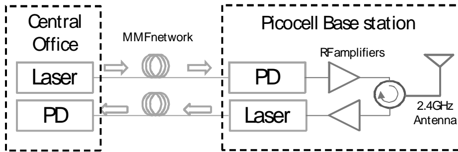
Fig.11. Radio over multimode fiber using IM-DD for WLANs.
