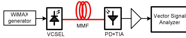
Fig. 14. Measurement setup for WiMAX over MMF.
