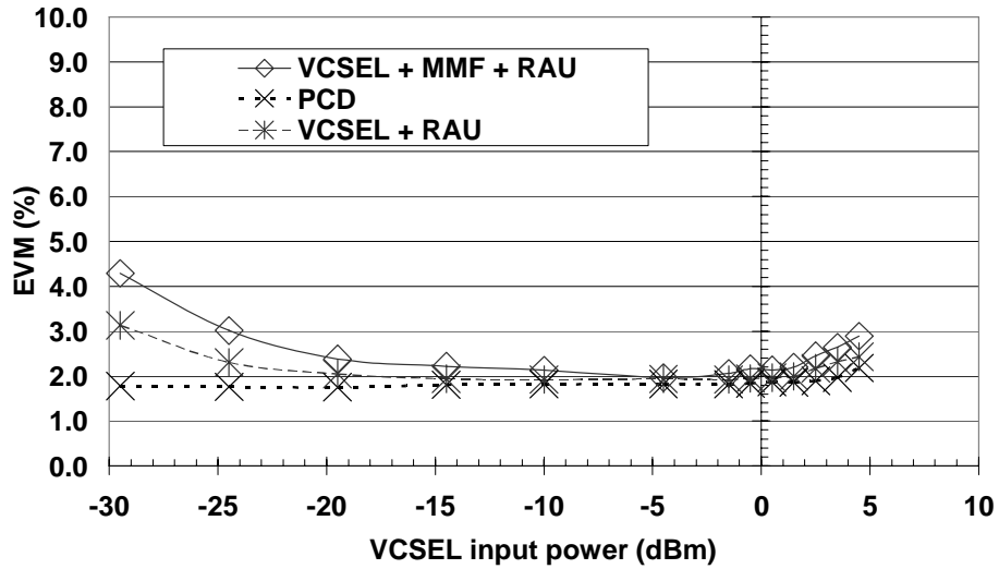
Fig. 17. EVM measurements for downlink UMTS radio over fiber transmission in the system of Fig. 16, as a function of central unit VCSEL RF drive power. Note: all other systems are present. [13].
