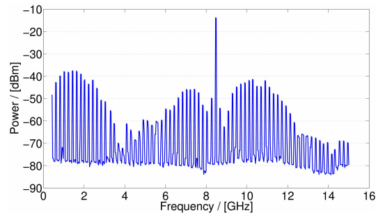
Fig.5. Measured up-converted spectrum at the output of the fiber link. The monocycle is present at baseband and around the local oscillator at f_{\text{LO}}=8.5 GHz.
