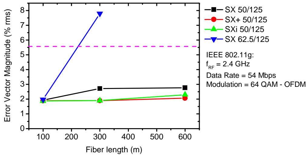
Fig.12. EVM measured as a function of fiber length [12].
