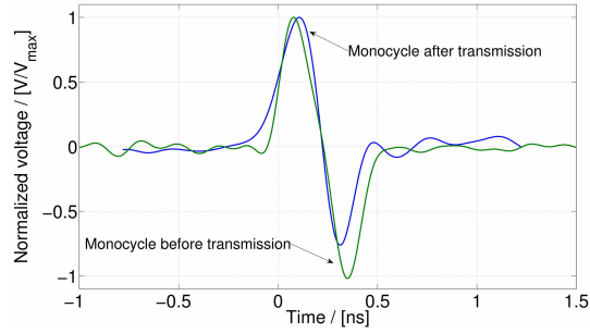
Fig. 6. Original base-band monocycle and after up-conversion at 8.5 GHz , I_{bias}=3 mA.
