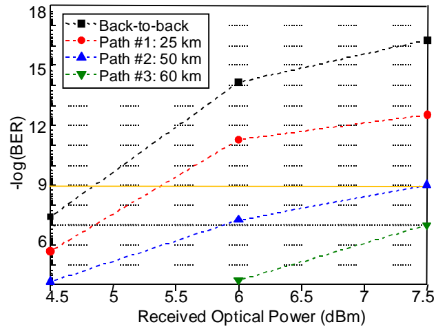
Fig.3. IR-UWB BER vs optical power for different RoF SSMF paths.
