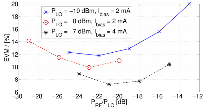
Fig. 10. Measured EVM after up-conversion to f_{RF} + 2f_{LO} = 5.1 GHz as a function of the power ratio P_{RF}/P_{LO} between the RF signal and the local oscillator
