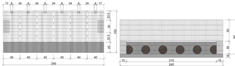
Figure 1: Top view and front view of collective pens. Distances in cm.
