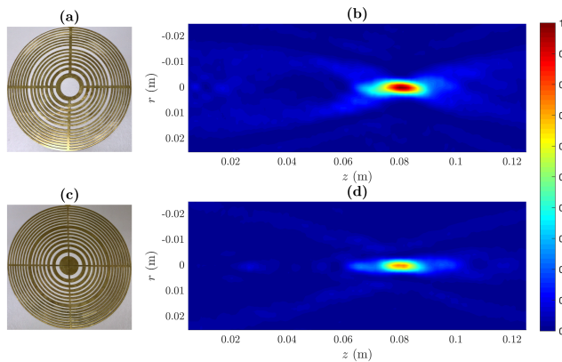
FIG. 4: Experimental results: (a) T-FZP and (b) its measured intensity map, (c) O-FZP and (d) its measured intensity map.
