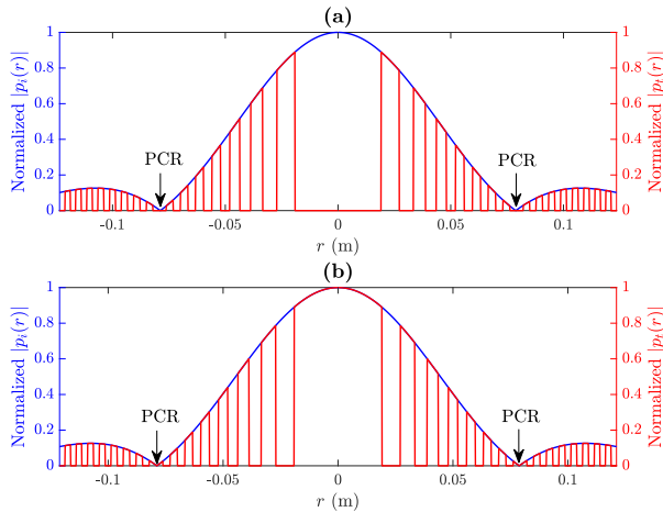
FIG. 1: Incident (blue line) and transmitted (red line) acoustic pressures in: (a) O-FZP, (b) T-FZP.
