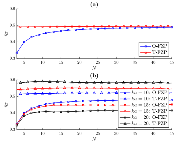
FIG. 2: Transmission efficiency: (a) plane wave incidence and (b) directional transducer placed at d = 340 mm from the lens.
