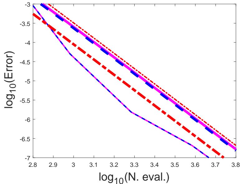
Figure 4: RKN methods of order 4(3) . Same as Figure 3 for the following methods: \mathcal{S}_643 (dashed lines); \text{eRKN}_443 (dot-dashed lines); and \mathcal{RKN}_643 (solid lines).
