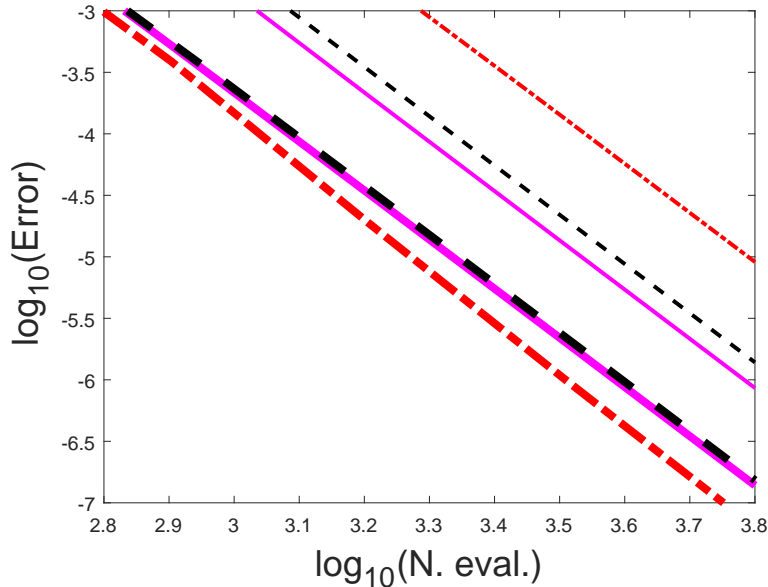
Figure 3: General methods of order 4(3) . Comparison of the true error (thin lines) and the estimator (thick lines) for e = 1/2 and the following schemes: \mathcal{PRK}_643 (dashed lines); e\mathcal{PRK}_543 (dot-dashed lines); and \mathcal{SS}_543 (solid lines).
