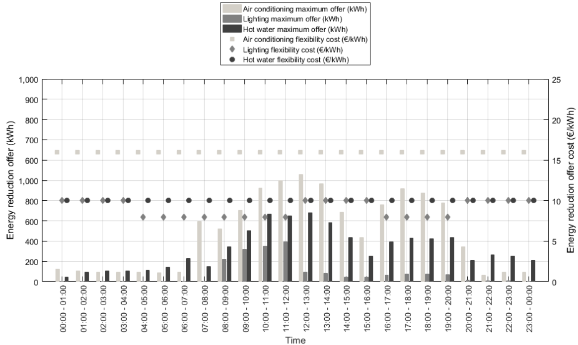
Figure 3. Offers of maximum flexible demand curtailment in the CPI facilities during the most favourable day and its associated costs (for the day of the DRP, these values are used to evaluate the results).
