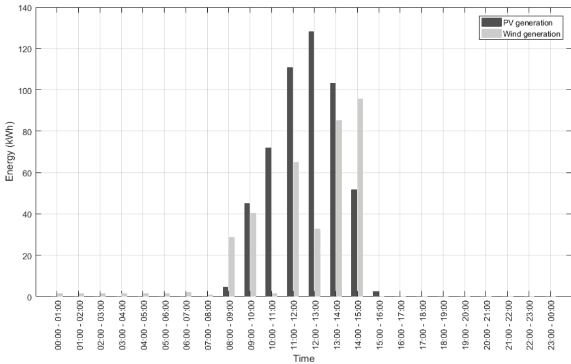
Figure 4. Generation curves obtained from real measurements in LabDER, used to simulate the optimal management during the proposed DRP.
