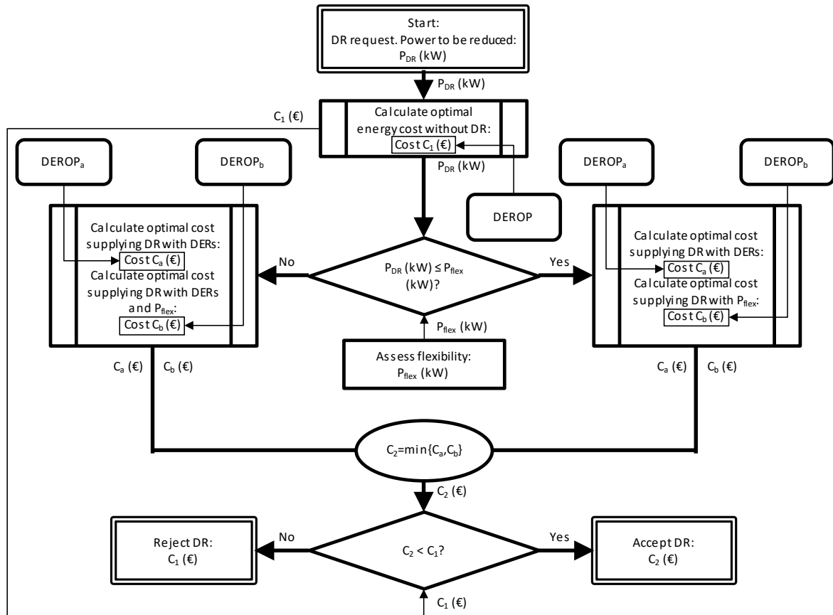
Figure 1. Flow diagram of DROP algorithm to optimise DR actions in facilities with DERs.
