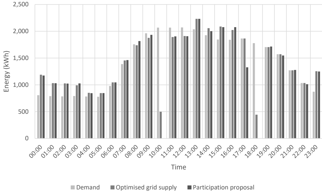
Figure 5. Electricity supply from the grid during the day of the DRP optimised with DEROP, demand to meet and optimised participation proposal using DROP.
