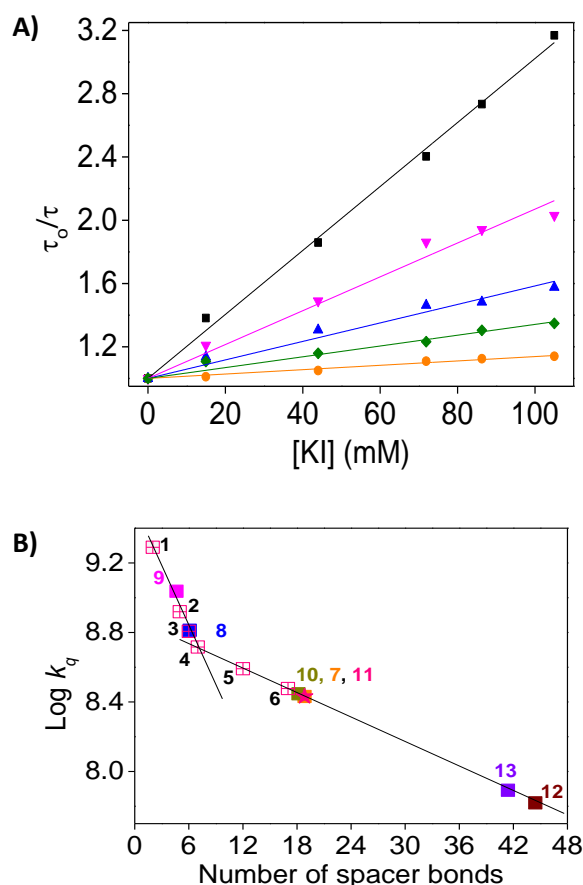
Fig 5 A) Stern-Volmer plots obtained for the time-resolved iodide fluorescence quenching of 1, 7, 8, 9 and 10 ; B) Plots of the quenching rate constants (Log k_q ) vs “number of spacer bonds” together with the data found from 1 to 6 (blank squares) used to build-up the bathymeter as shown in Figure 3B. All data were obtained within MM containing the appropriate probe under time-resolved conditions.
