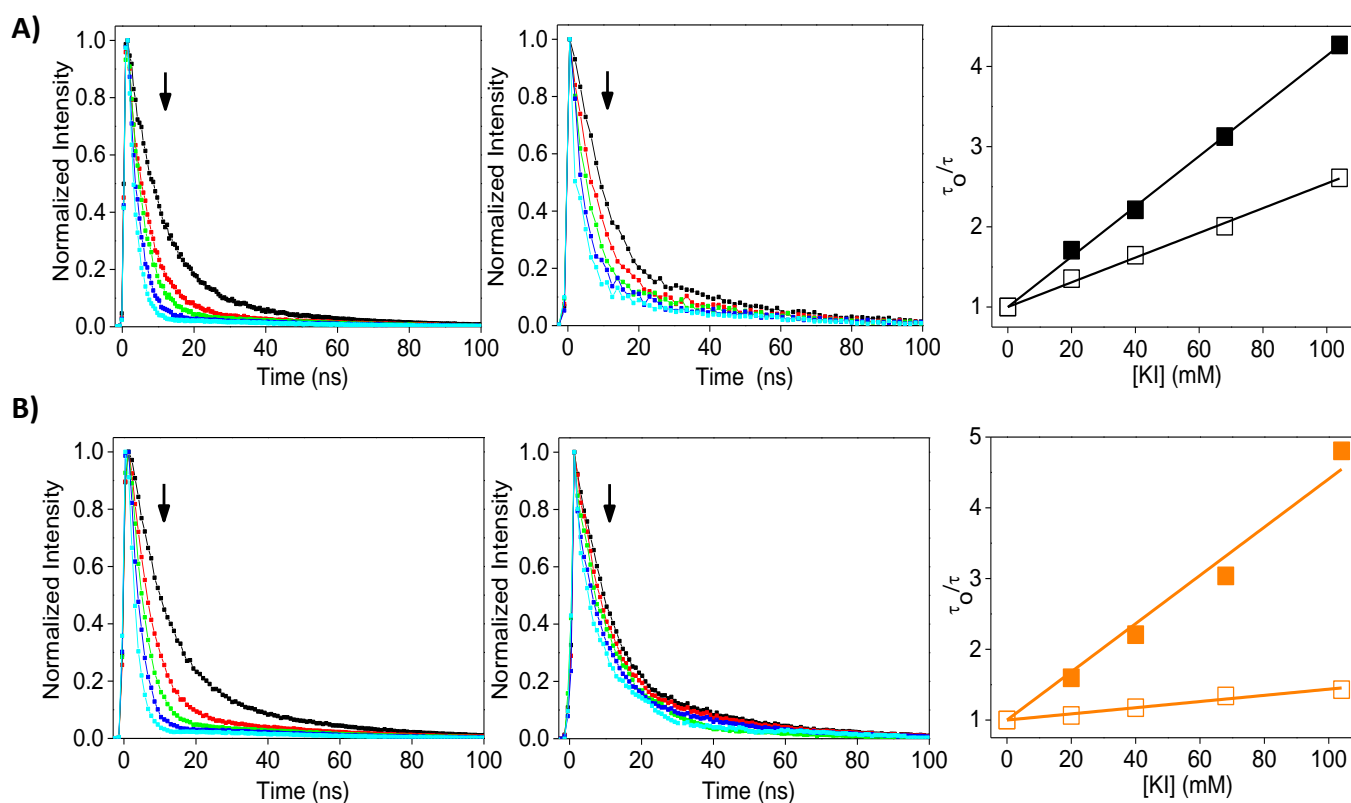
Fig. 2 Changes in the emission decay traces ( \lambda_{\text{exc}} = 295 nm) of 1 (A) and 6 (B) upon addition of increasing amounts of KI (0-104 mM), in aqueous NaCl 0.2 M (left) and inside MM (middle). Right column: corresponding Stern-Volmer plots in solution (solid squares) and in MM (blank squares).
