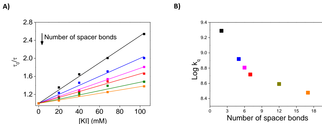
Fig. 3 A) Stern-Volmer plots obtained for the iodide fluorescence quenching of the photoactive derivatives; B) Plots of the apparent quenching rate constants ( \text{Log } k_q ) vs number of spacer bonds. All the experiments were run within MM containing the appropriate probe (1, 2, 3, 4, 5 and 6) under time-resolved conditions.
