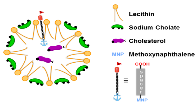
Fig. 1 Cartoon representation of the photoactive probes with different spacer lengths anchored to the surface by the acid while keeping the chromophore diving as far as allowed inside MM.
