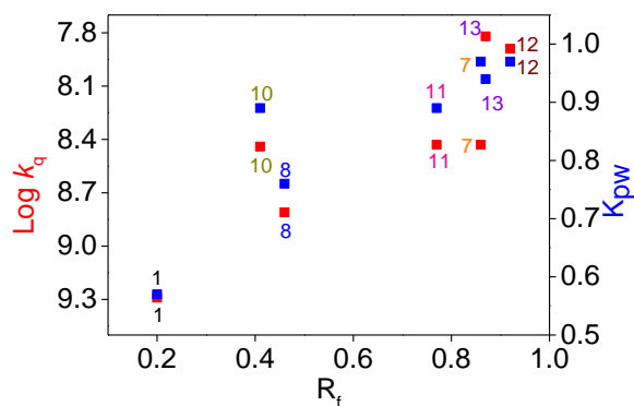
Fig 6 Dynamic rate constants for iodide fluorescence quenching ( \text{Log } k_q , Left) and partition coefficient, pentane:water ( K_{pw} , Right) versus R_f , for 1 , 7 , 8 , 10 , 11 , 12 and 13 .
