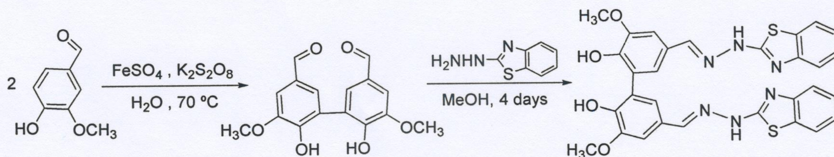
Scheme 1. Synthesis of L.
