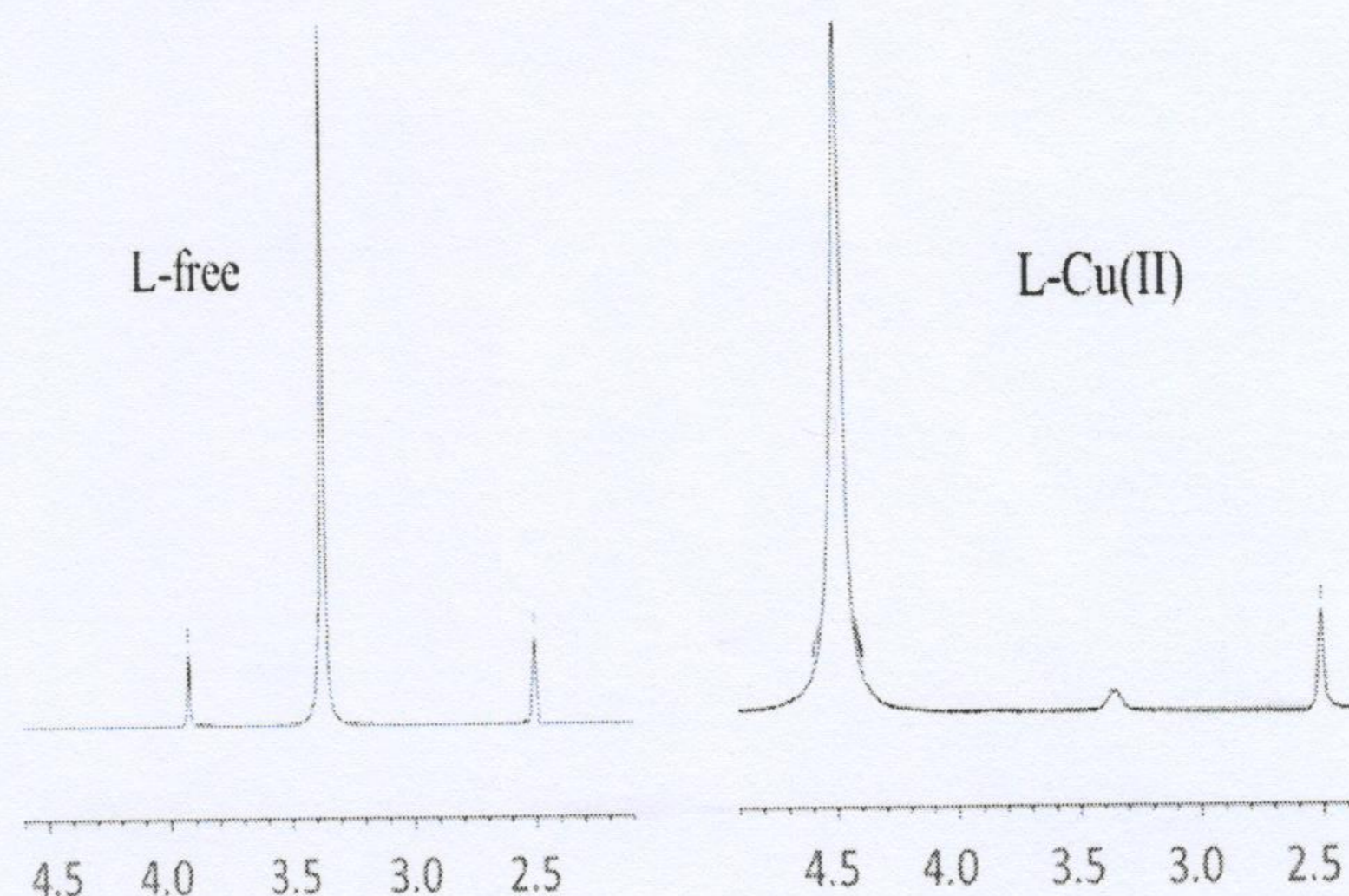
Figure 4. 1 H NMR spectra of L (in DMSO-d 6 ) and L-Cu 2+ (DMSO-d 6 :D 2 O 1:1) and fitting to 1:1 complex model.
