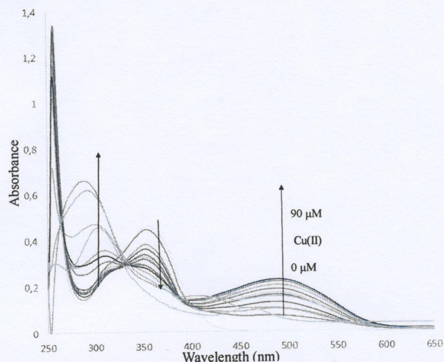
Figure 3.a. UV-vis titration spectra of L (10 \mu\text{M} DMSO) when different amount of Cu 2+ were added.
