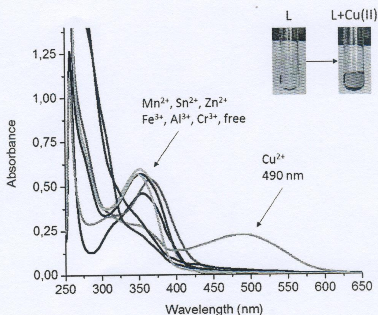
Figure 1. UV-vis absorption spectra of L with \text{Cu}^{2+} and other metal ions (inset: visual colour change with \text{Cu}^{2+} ).
