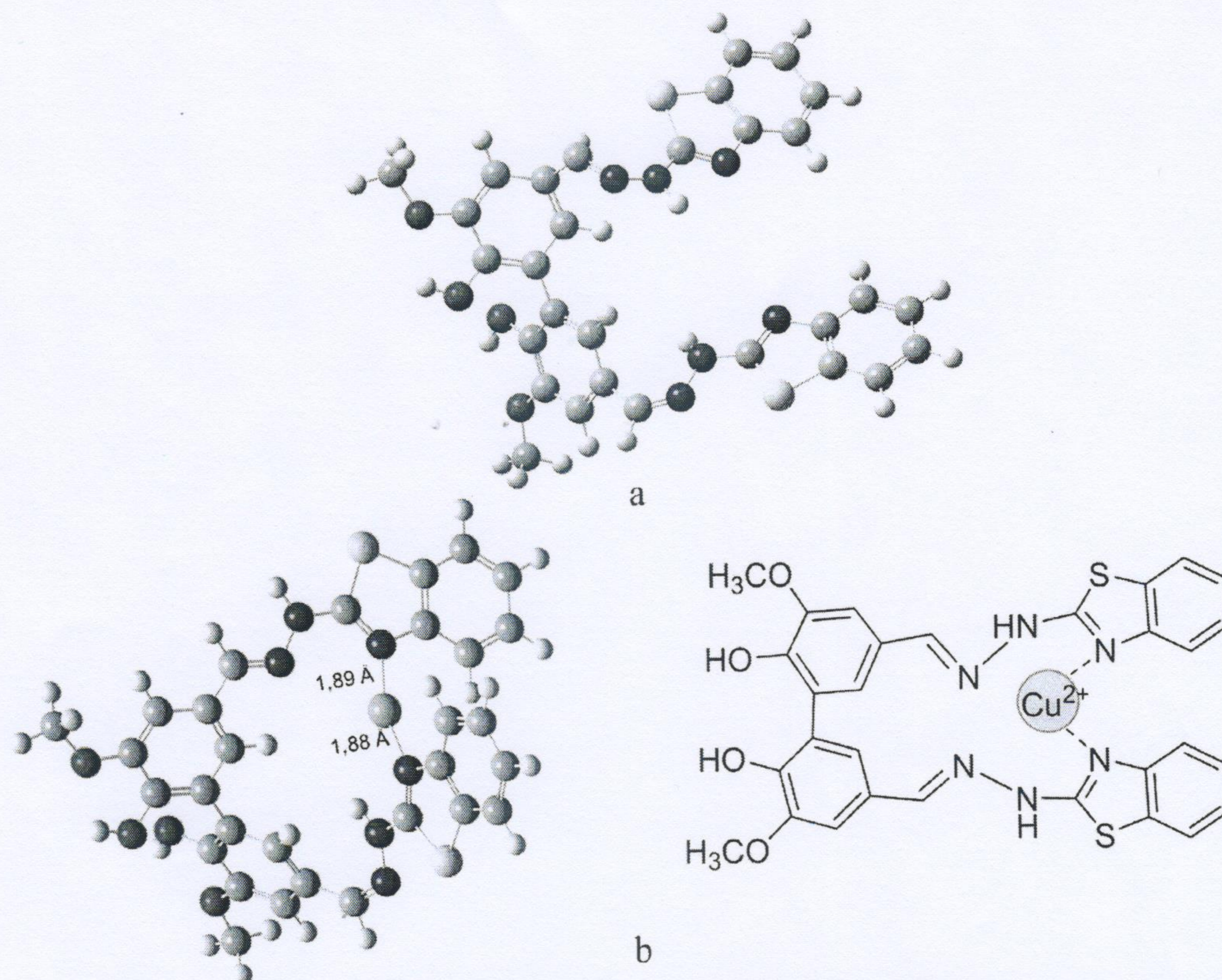
Figure 5. Optimized structures of L (a) and L-Cu 2+ complex (b). The dihedral angle for L and L-Cu 2+ are 59,53° and 48,41°, respectively.
