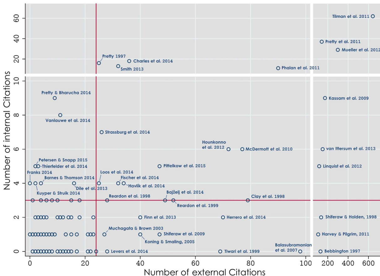
Fig. 3. Relationship of external and internal citations in the analysed literature. Based on Scopus database and citation records (N = 330). Two additional solid (red in web version) lines represent the 90% quantiles of the respective axes. The citations of 194 articles do not exceed both quantiles. 96 papers are not cited and, therefore, excluded. Source: Own representation.
