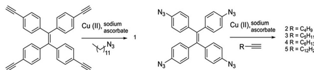
Scheme 1 Synthesis of compounds 1–5.
