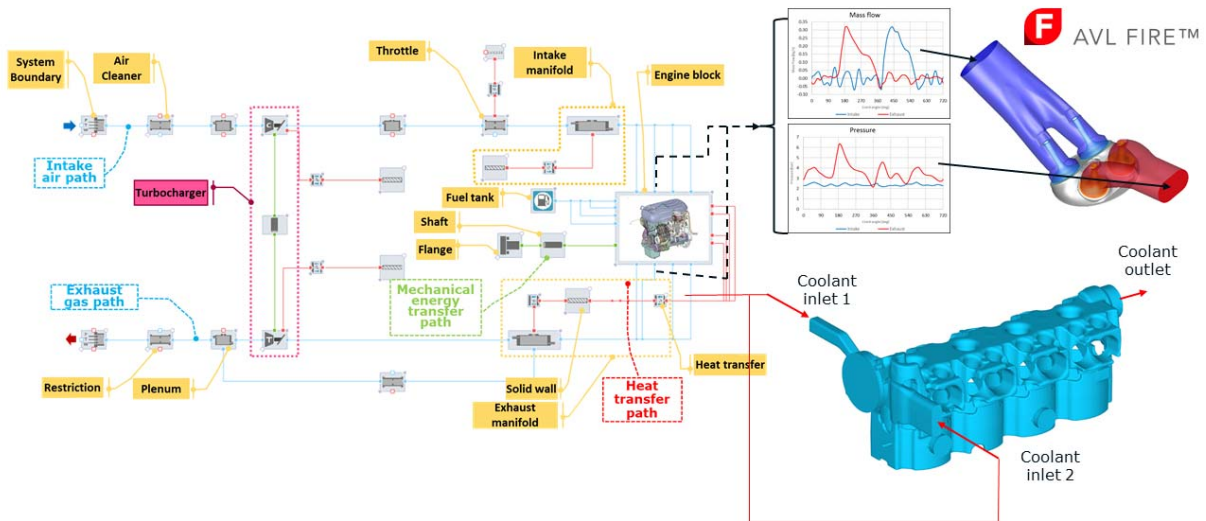
Fig. 3. Engine model
