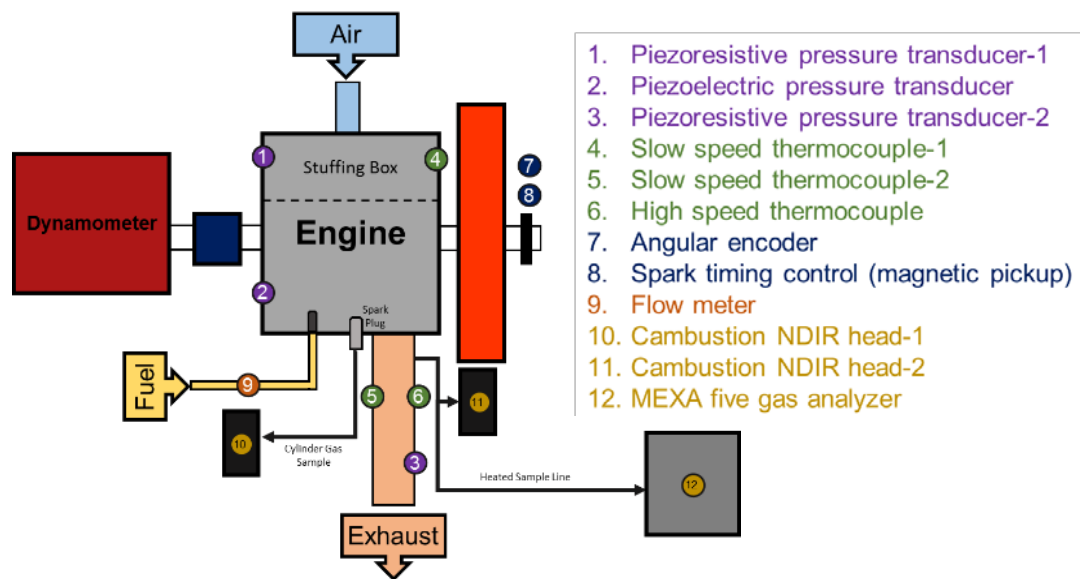
Fig. 2. Test bed schematic with all available sensors labelled
