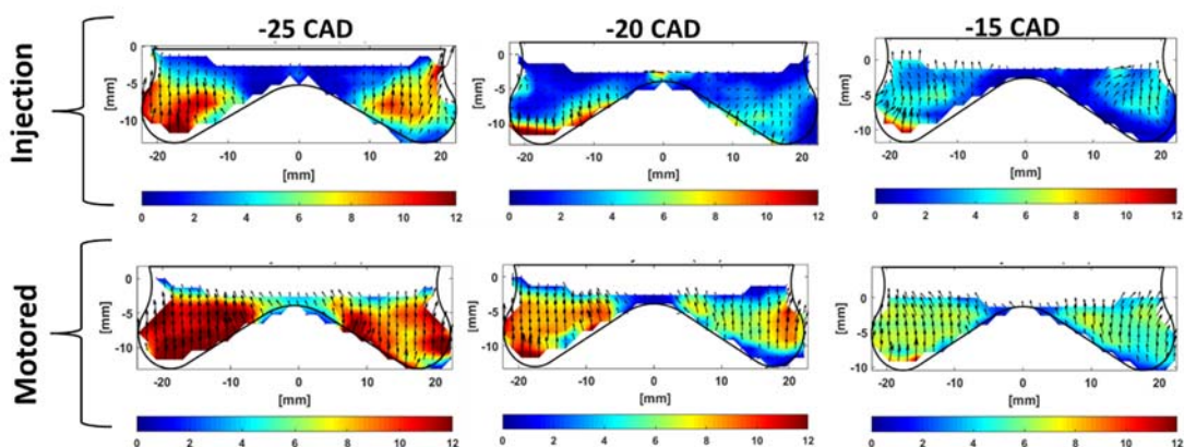
Fig. 7- Mean flow velocity field at motored and injection conditions
