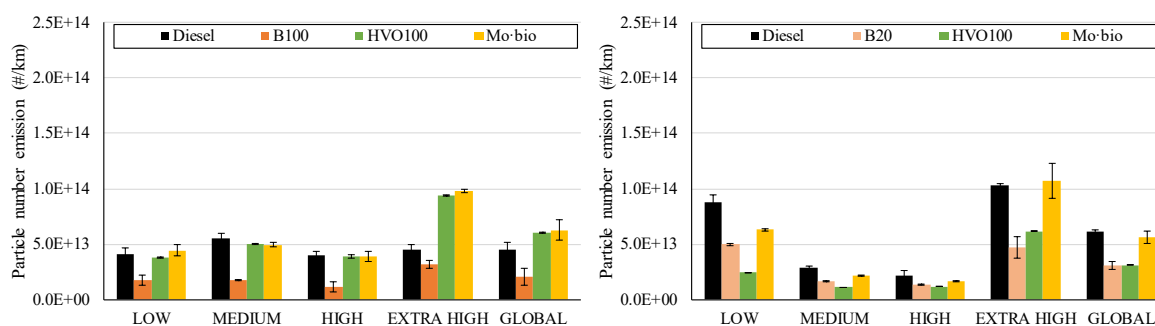
Fig. 15. Specific particle number emissions at 24^\circ\text{C} (left) and -7^\circ\text{C} (right)
