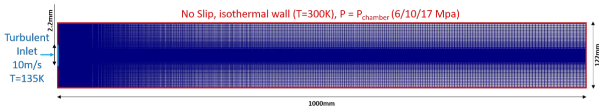
Fig. 2. Dimensions of the cylindrical chamber along with the boundary conditions implemented and the cut section of the mesh
