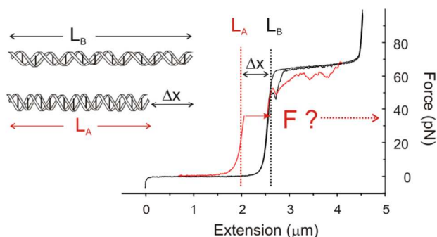
Fig. 6 Hypothesis of a force-induced A \rightarrow B transition. A dsDNA molecule in high alcohol concentration and/or with a high G•C content switches from the A to the B form at a force F (red curve). As a reference of the B-form elastic behaviour, the previous stretch-relaxation cycle of the pBACgus11 DNA molecule (Fig. 4), stable in B-form in aqueous buffer solution, is plotted in black.
