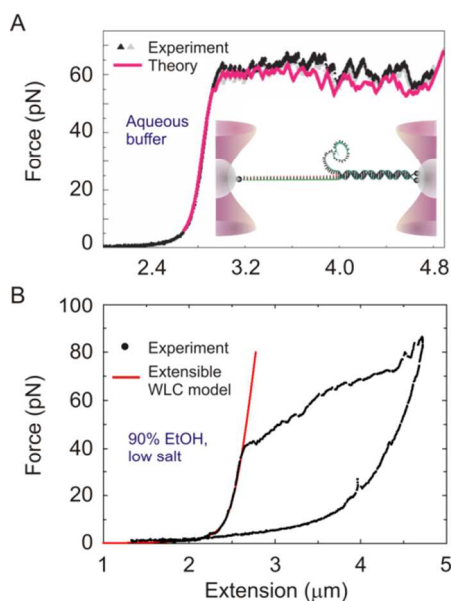
Fig. 5 Force-induced unpeeling of dsDNA. A duplex, held between two beads by only one strand in one of its ends, is melted from the free strand end as depicted in the inset of A. (A) Force-extension curve of an 8.4-kbp molecule (pKYB1 plasmid) taken at 10 nm/s in physiological conditions (50 mM NaCl, 10 mM Tris-HCl, pH 7.8, 20°C). The overstretching plateau reveals a sequence-dependent stick-slip dynamics. Reproduced from 111a with permission, copyright (2011) Macmillan Publishers Ltd. (B) Force-extension curve of an 8.0-kbp molecule (pBACgus11) taken at 500 nm/s and 20°C in a mixture of 90% ethanol with 1 mM NaCl TE buffer (10 mM Tris-HCl, 1 mM EDTA, pH 7.5). In this case, unwinding and unpeeling processes meet in an “overstretching transition” that is no-longer a plateau. The molecule relaxes as ssDNA as a consequence of the low polarity solution. A fitting to the so-called Worm-like chain (WLC) model reveals a persistence length and stretch modulus dramatically lower than in physiological conditions ( P = 13.7 nm, S = 878 pN) due to the presence of ethanol. Reproduced from 111b with permission, copyright (2012) Wiley Periodicals, Inc.
