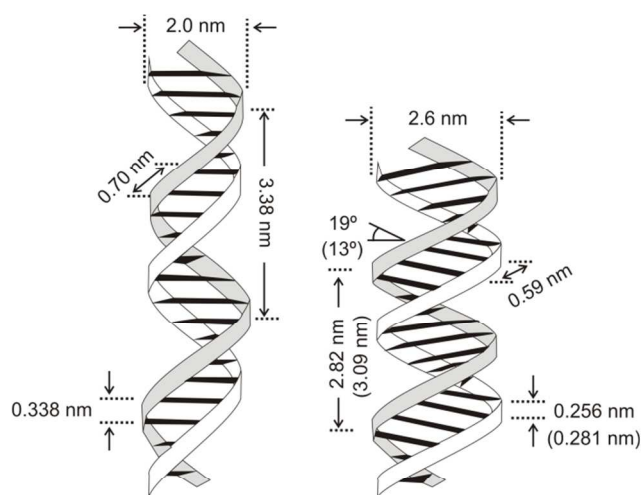
Fig. 1 Schematic view of the B (left) and A (right) double-helix forms. Structural parameters are approximate, based on sequence averages and in the absence of force. Some of them are slightly different for the A-form in dsRNA (in brackets) with respect to that in dsDNA. Helix diameters have been estimated from the dislocation data in 6 . Base-pair tilts are negative and much smaller for B-DNA than for both A-DNA and dsRNA and therefore have not been represented in the left diagram.
