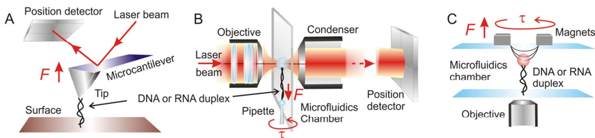
Fig. 3 Basic elements of the most used single-molecule mechanical manipulators. (A) AFM, a type of scanning probe microscopy that consists of a micro-cantilever ending in a nanometre-scale tip. A polymer can be stretched between the tip and a surface and the forces measured by following the cantilever displacement via laser-beam deflection on a photodiode. (B) In optical tweezers, laser light is highly focused by a microscope objective and collected by a condenser lens. A microbead can be trapped in the focal region, which is produced inside a fluidics chamber. A micropipette inserted in the chamber can hold a second bead by suction. By translating and rotating the micropipette relative to the trap, a polymer can be stretched and twisted, respectively. The collected exiting rays are registered by a position-sensitive photodetector. (C) Conventional magnetic tweezers uses two small magnets to pull and rotate a magnetic microsphere inside a fluidics chamber. Here, the polymer is held between the microsphere and the bottom coverslip. A microscope objective is used to monitor the experiment.
