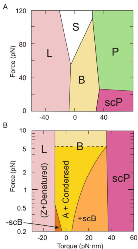
Fig. 11 DNA force-torque phase diagram near physiological conditions. Colour regions represent conditions for the stability of pure structures; lines indicate conditions for structural coexistence of two conformations in a single dsDNA molecule. (A) Early diagram adapted from 97 , copyright (2001) American Physical Society. (B) Phase diagram at low forces. Conditions for Z-DNA and A-DNA plus condensation often require high ionic strengths and/or polycations and low humidity. Revised from 119 and 96b with permission, copyright (2007 and 2011) American Physical Society, following these sources and the present review report. scP, supercoiled P-DNA; +scB and -scB, supercoiled B-DNA at overwinding and underwinding torques, respectively. Changes in ambient temperature, pH and salt type and concentration, which may modify coexistence lines and triple points, have not been considered in depth.
