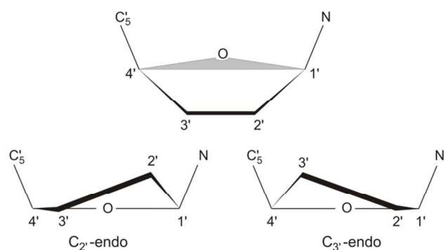
Fig. 2 Geometrical disposition of the atoms in the five-membered sugar into puckering modes. Top, starting position with flat conformation. Bottom left, C_2' -endo sugar-puckering mode in which the 2' carbon, whose bonds are not compromised to the backbone units, is raised north. This mode is observed in B-DNA. Bottom right, C_3' -endo mode in which the 3' carbon atom, the one that links adjacent bases through a phosphate group in the strand backbone, is raised north. This mode is observed in dsRNA and in A-DNA. In reality, C_2' -endo and C_3' -endo modes consist of two each families of closely related puckering modes. 6 Mechanical tension may cause continuous transitions within a puckering family because their states lack of substantial potential energy difference. Transitions C_2' \leftrightarrow C_3' are however energetically less probable.
