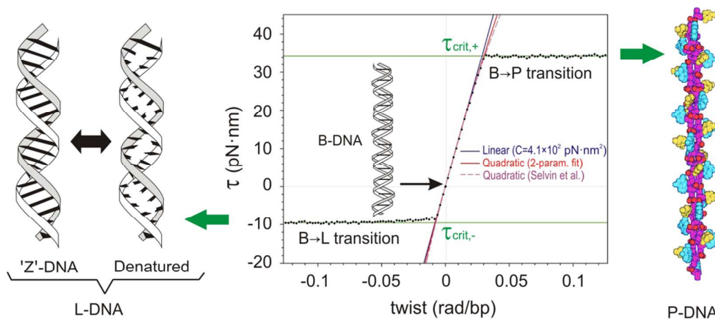
Fig. 10 Torque-twist characterization of dsDNA. The central diagram shows a torque-angle curve at constant tension; different forces generate similar curves according to the force-torque diagram of Fig. 11. Reproduced from 71 with permission, copyright (2003) Macmillan Publishers Ltd. The left schematic depictions address the two mixed phases that can take place at underwinding torques, the Z-like ('Z') DNA and the denatured phase, which, apart from environmental conditions, depend on sequence. The right figure is a molecular model of P-DNA, which takes place at overwinding torques. Reproduced from 13a with permission, copyright (1998) National Academy of Sciences, U.S.A.
