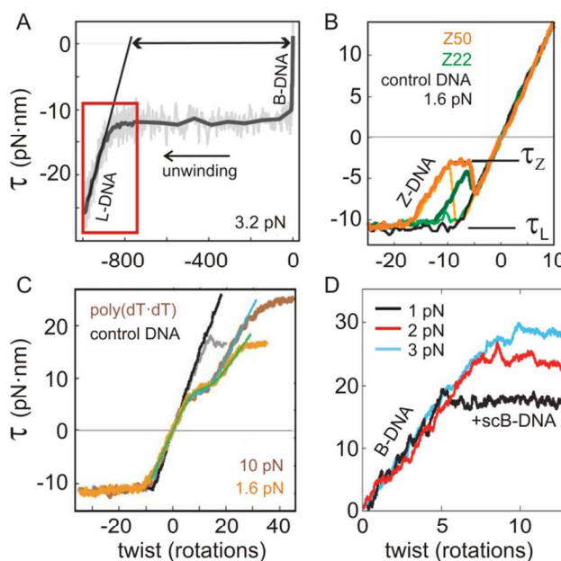
Fig. 12 Torque-twist curves of dsDNA at low force. (A) B-L transition of a 4.6-kbp control dsDNA molecule. (B) B-Z transition of either a 50-bp or a 22-bp long GC-insert molecule in a PBS (phosphate buffered saline) solution (137 mM NaCl, 2.7 mM KCl, 0.5 mg/mL BSA, 10 mM Na 2 HPO 4 , 2 mM KH 2 PO 4 , 5 mM EDTA, pH 7.4). (C) B-to-denatured DNA transition for a 100-bp insert with mismatched dT bases in the same PBS solution. (D) B-scB (positively supercoiled B-DNA) transition of a 2.2-kbp dsDNA molecule in 150 mM NaCl PBS solution, 23.5°C. (A-C, reproduced from 12 with permission; D, reproduced from 101 with permission, copyright (2008) American Physical Society).
