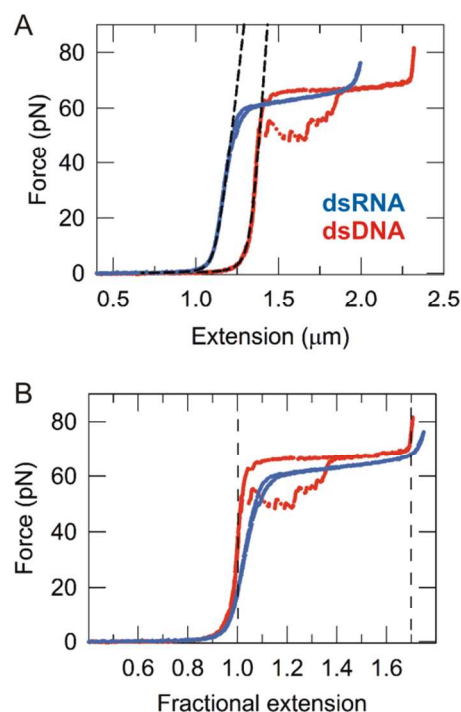
Fig. 7 Force–extension characterization of dsRNA and dsDNA substrates of equivalent sequence. (A) Force–extension curves in 10 mM Tris-HCl with 300 mM NaCl and 1 mM EDTA (pH 8.0). Stretch–relax cycles were performed at 500 nm/s. Blue and red dots correspond to data points of a dsRNA and a dsDNA molecule, respectively, with their corresponding fittings, black dashed curves, to the extensible WLC model. The fits for these examples yielded values of (contour length) L = 1.14 \mu\text{m} , (persistence length) P = 59.8 \text{ nm} , and (stretch modulus) S = 632 \text{ pN} for dsRNA and L = 1.36 \mu\text{m} , P = 48.5 \text{ nm} , and S = 1280 \text{ pN} for dsDNA. (B) Same as in (A) with extension axis of each substrate molecule normalized to its respective contour length. Dashed lines at fractional extensions 1.0 and 1.7 demarcate the elasticity regimes. Adapted from 18 with permission, copyright (2013) American Chemical Society.
