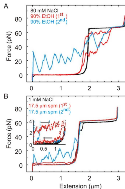
Fig. 9 Condensation of a single DNA molecule under force. In each graph, a single molecule of dsDNA (piJ702 plasmid, 5682 bp, 70% G•C content) is first stretched and relaxed in physiological buffer (black curve), followed by two successive stretch/relax cycles (red and blue curves) in a buffer-90 % ethanol mixture (A) or in buffer with a low concentration of spermine (B). Reproduced from 11c with permission from Elsevier, copyright (2011).
