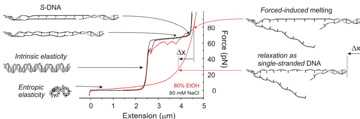
Fig. 4 Force-extension characterization of dsDNA. The graph shows an individual DNA molecule from pBACgus11 plasmid (8022 bp, 48% G•C), first stretched and relaxed in 80 mM NaCl, 10 mM Tris-HCl, 1 mM EDTA, pH 7.5 (black line), and subsequently stretched and relaxed in a mixture of the same buffer with 80% ethanol (red line). Pulling speed, 500 nm/s. The lateral schemes illustrate the strands arrangement as a function of the pulling/relaxing force according to the literature (see text for details).
