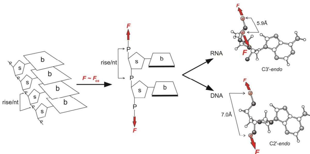
Fig. 8 Schematic depiction of the elastic response of nucleic acids under force. Rise per nucleotide (rise/nt) depends on the stacking of bases ( b ) in the absence of stress. When force is applied at overstretching values ( F \approx F_{os} ), bases unstack and rise per nucleotide is restricted by the distance between phosphates linking adjacent sugar rings ( s ), which is of 5.9 Å in dsRNA, where sugar rings are in C_3' -endo conformation, and of 7.0 Å in dsDNA, where they adopt the C_2' -endo conformation. Reproduced from 18 with permission, copyright (2013) American Chemical Society.
