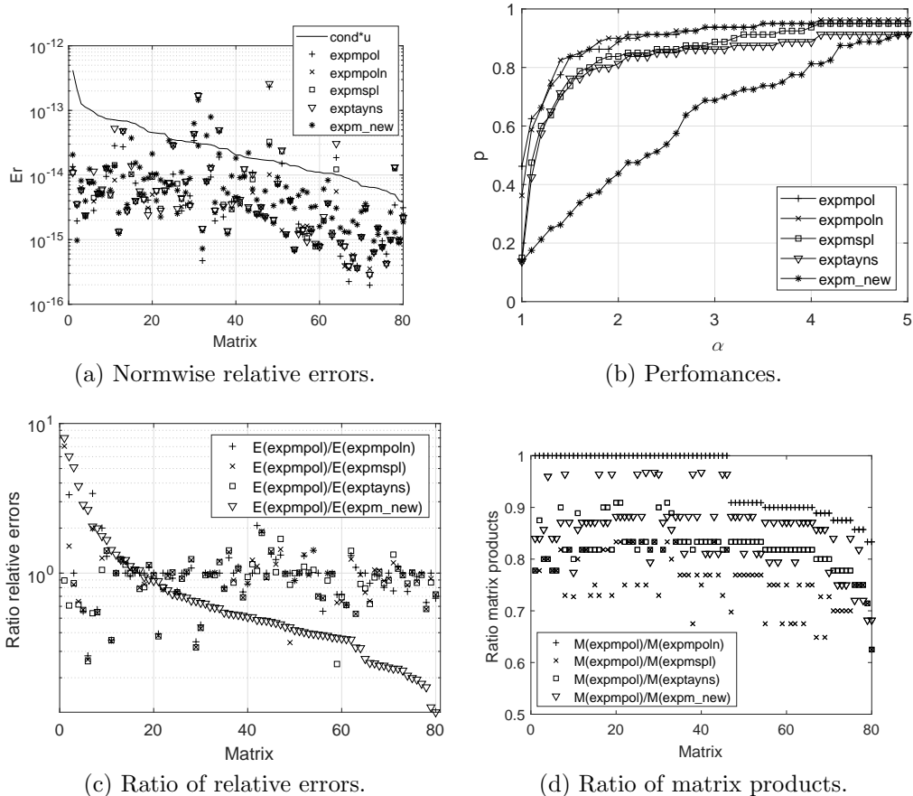
Figure 2: Experimental results with Test 2. All the Taylor functions use maximum order m_M = 30 .
