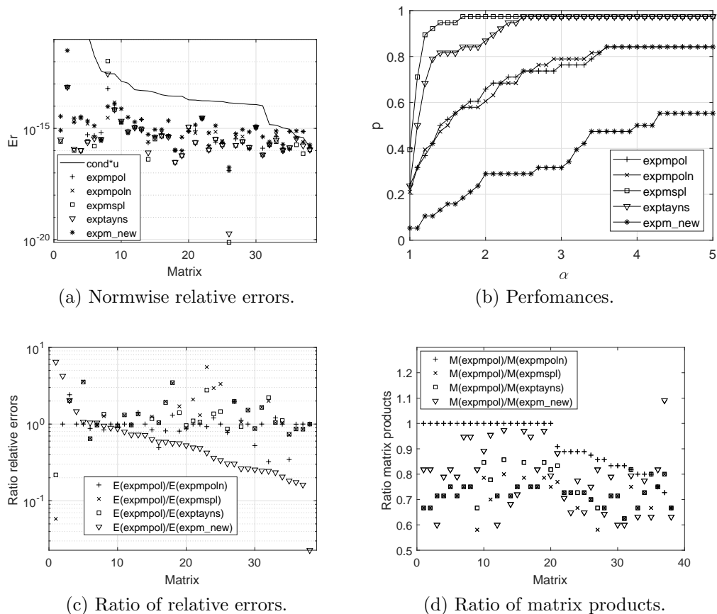
Figure 4: Experimental results with Test 3: \text{expmpol} and \text{expmpol} with m_M = 24 , \text{exptayns} with m_M = 25 and \text{expmspl} with m_M = 30 .
