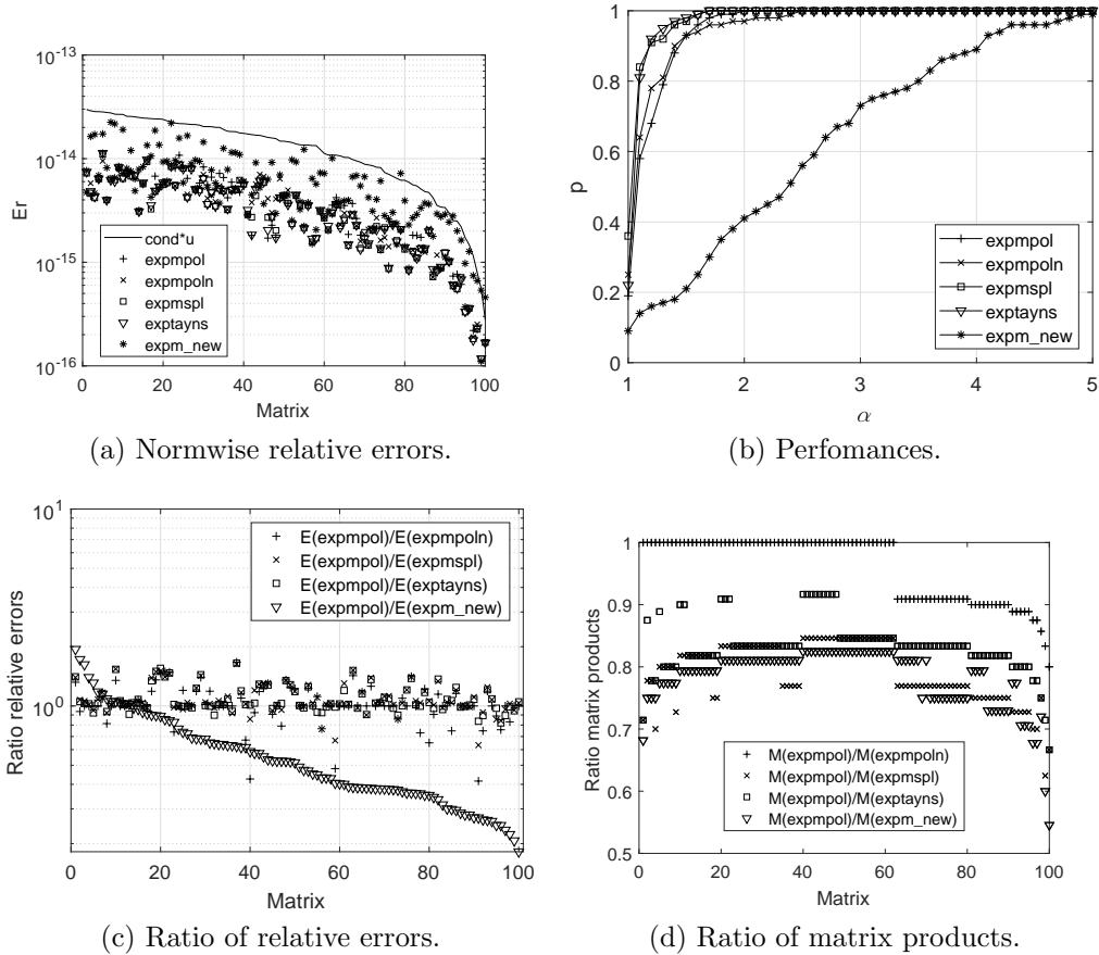
Figure 1: Experimental results with Test 1. All the Taylor functions use maximum order m_M = 30 .
