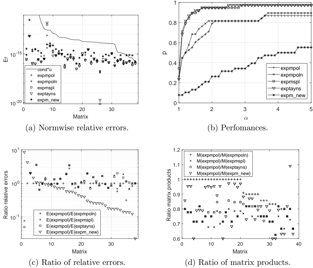
Figure 3: Experimental results with Test 3. All the Taylor functions use maximum order m_M = 30 .
