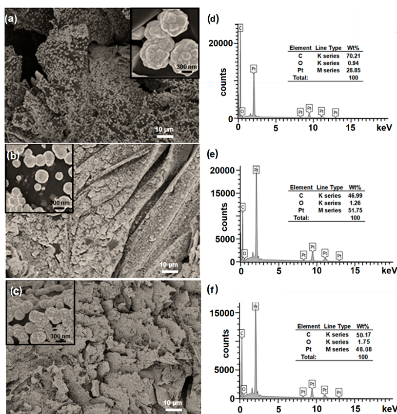
Figure 5. (a–c) Micrographs of GFE/Pt ( E_i = 0.20 V), GFE/RGOPt ( E_i = 0.20 V), and GFE/RGOPt 50 at magnifications Mag = 500 \times . Insets: The same but at Mag. = 20.00 K X. (d–f) EDX analyses of GFE/Pt ( E_i = 0.20 V), GFE/RGOPt ( E_i = 0.20 V), and GFE/RGOPt 50 , respectively. For EDX, a 500 \times 500 \mu m surface was scanned.
