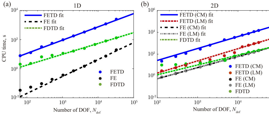
Figure 8: Computation time as a function of number of degrees of freedom for (a), 1D, \mathbf{k} = \pi/a , and (b), 2D, \mathbf{k} = (\pi/2a, \pi/2a) . Circles represent the computation time results obtained directly from numerical simulations and lines represent curve fits of this data using the expression \bar{y} = a\bar{x}^b . Note that the number of DOF used for the calculations presented in Figs. 2 and 3 are N_{\text{dof},1\text{D}} = 256 , N_{\text{dof},2\text{D}} = 2,048 , respectively.
