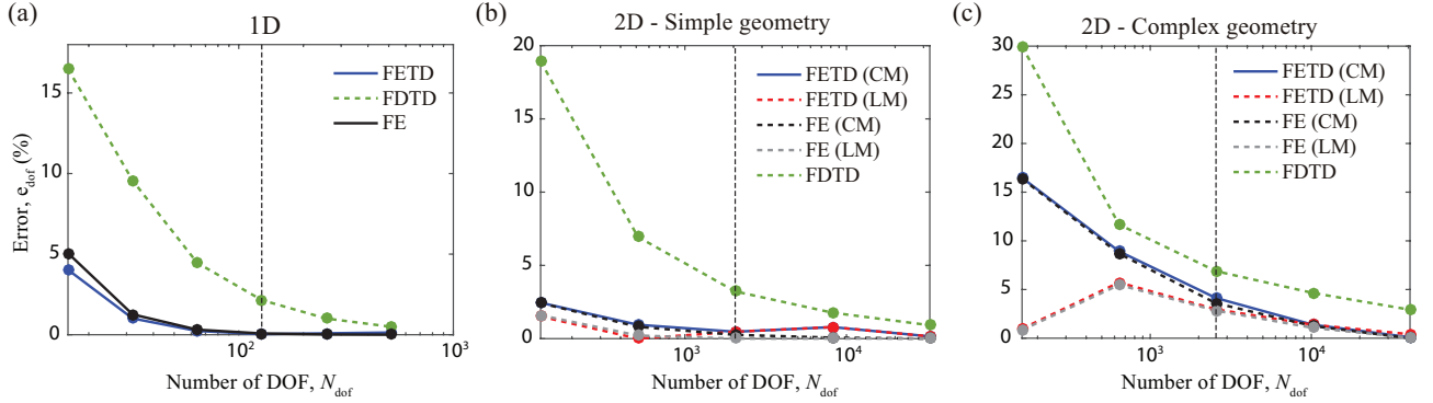
Figure 7: Frequency error estimation as a function of number of DOF for (a) 1D, \mathbf{k} = \pi/a , (b) 2D simple geometry, \mathbf{k} = (\pi/2a, \pi/2a) , and (c) 2D complex geometry, \mathbf{k} = (\pi/2a, \pi/2a) . Results are shown for the 4th branch. Vertical dashed black lines in the three subfigures mark the number of DOF used in Fig. 2 and Figs. 4 and 5, which are n_{\text{dof},1\text{D}} = 256 , and n_{\text{dof},2\text{D}} = 2,048 for the simple geometry and n_{\text{dof},2\text{D}} = 2,560 for the complex geometry. The reference method is high-resolution FE eigenvalue analysis using consistent mass matrices.
