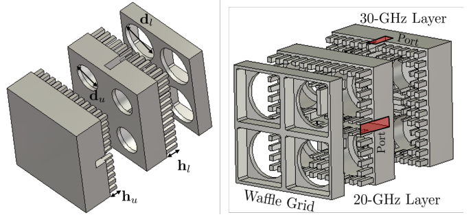
Fig. 3: Layers of the dual-band basic cell.
