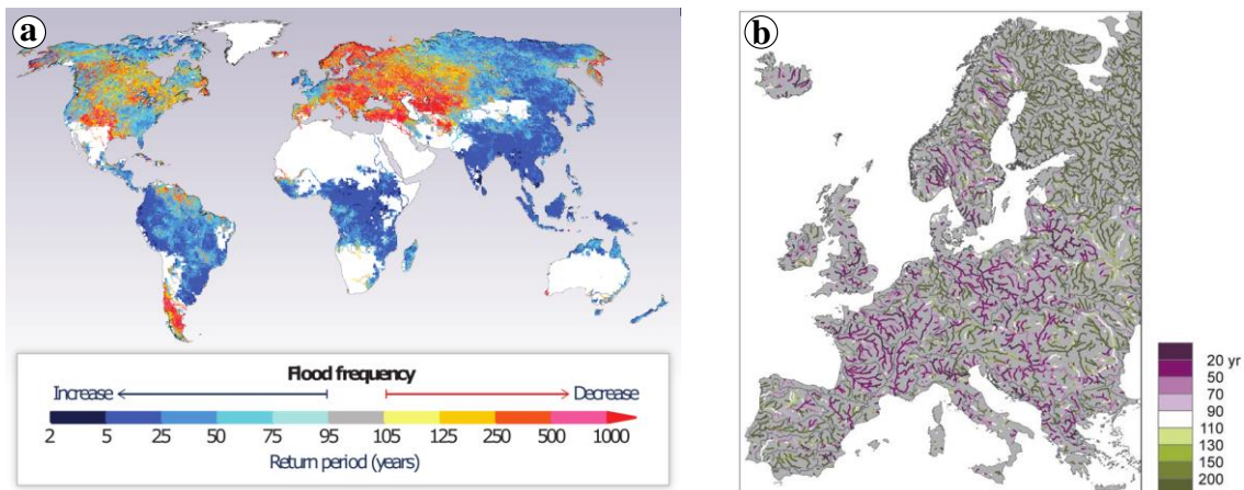
Figure 2-3. (a) Multi-model median return period (years) in the 2080s for the 20th century 100-year flood based on one hydrological model driven by 11 GCMs under RCP8.5 (from Hirabayashi et al. (2013)). (b) Change in recurrence of a 100-year flood in Europe in the H12A2 scenario run using a Gumbel distribution (from Dankers and Feyen (2008)).
