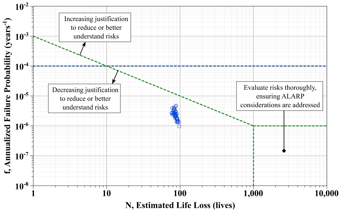
Figure 5-4. USBR tolerability criteria and f - N points representing the estimated failure probability and loss of life based on the risk results for 2019 (present).
