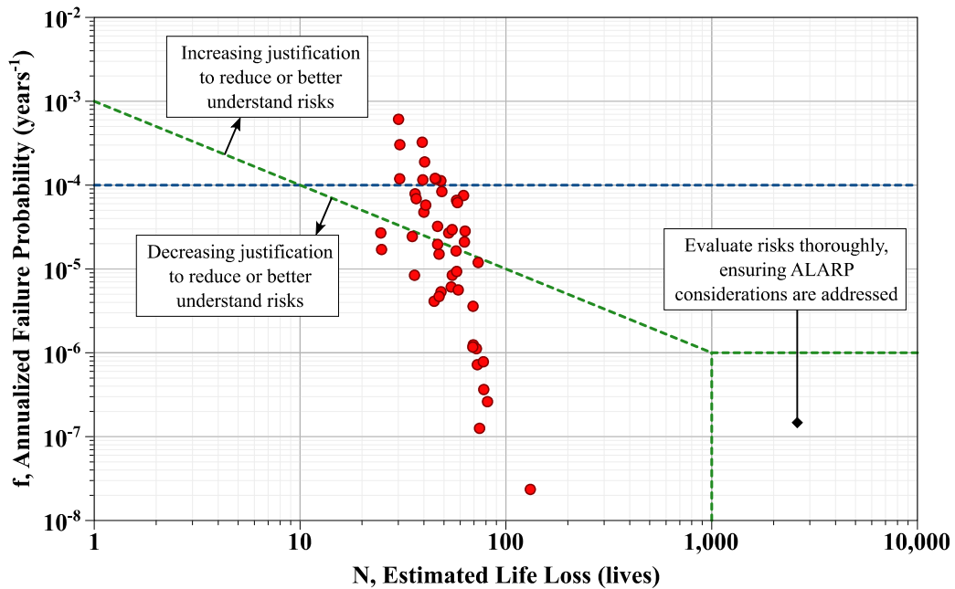
Figure 5-5. USBR tolerability criteria and f - N points representing the estimated failure probability and loss of life based on the risk results for 2059.
