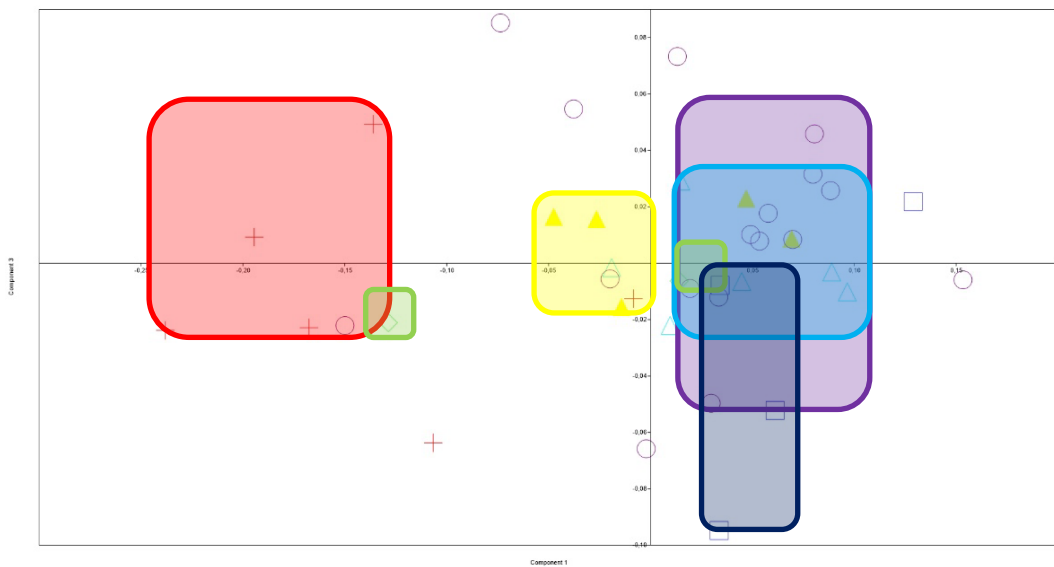
Fig. 3.6 PC1vs PC3 (Log) Box Color - Dental Metrics
