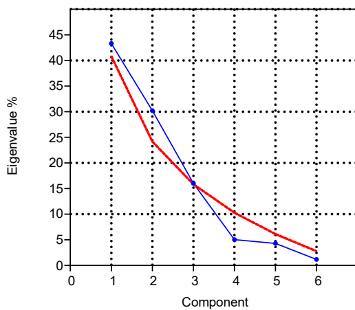
Fig. 3.17 PCA Scree Plot with Broken Stick (in red) - Sicilian Sample
