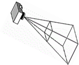
Fig. 2.9b Chunk1-Height2
