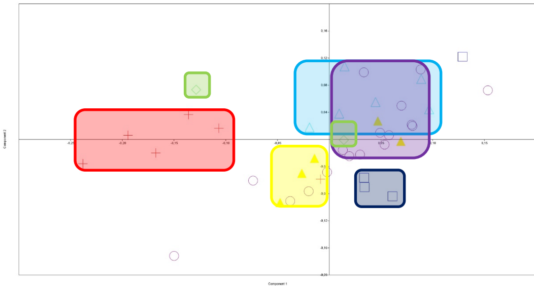
Fig. 3.5b PC1vs PC2 (Log) BoxColor - Dental Metrics
