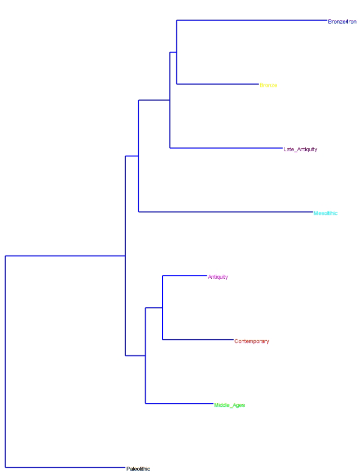
Fig. 3.15 Procrustes Coordinates Neighbour-Joining hierarchical tree representing the historical divergence among the Sicilian populations from Paleolithic to Contemporary
