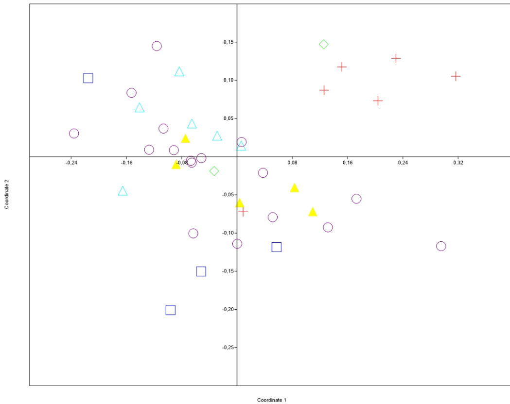
Fig. 3.10a MDS - Dental Metrcs
