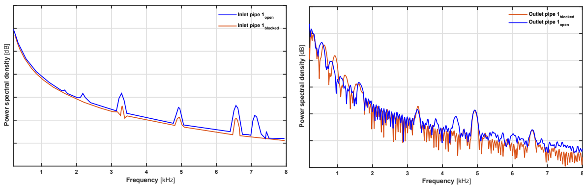
Figure 15: Experimental (top) and numerical (bottom) spectra of inlet (left) and outlet (right) ducts for open (blue) and blocked (orange) compressor configurations operating at design conditions.
