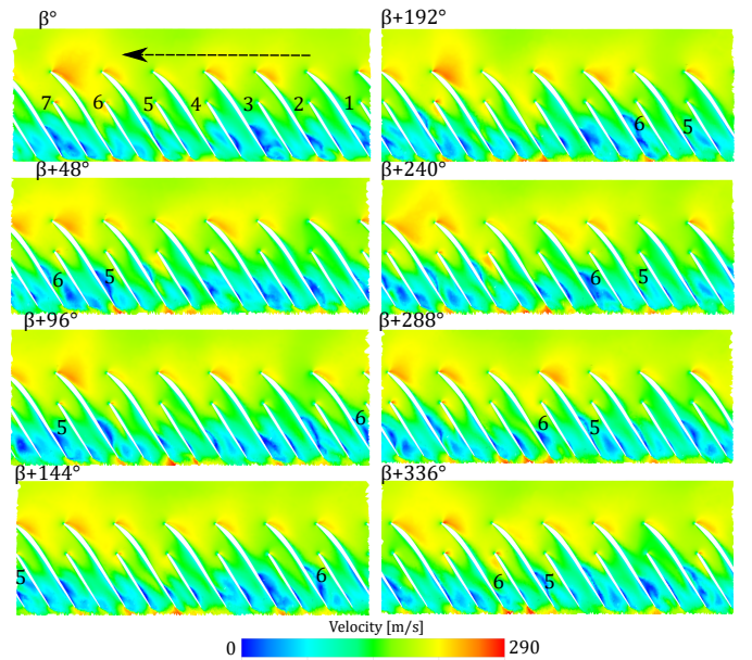
Figure 8: Instantaneous velocity distribution at impeller midspan for approximately one compressor revolution.
