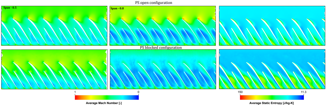
Figure 9: Blade-to-blade views of average Mach number distribution for 0.5 (left) and 0.8 (middle) blade span and average entropy generation (right) at 0.5 blade span for open (top) and blocked (bottom) compressor configurations operating at near surge conditions.
