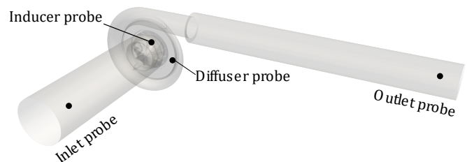
Figure 2: Computational domain along with the location of various virtual pressure probes.
