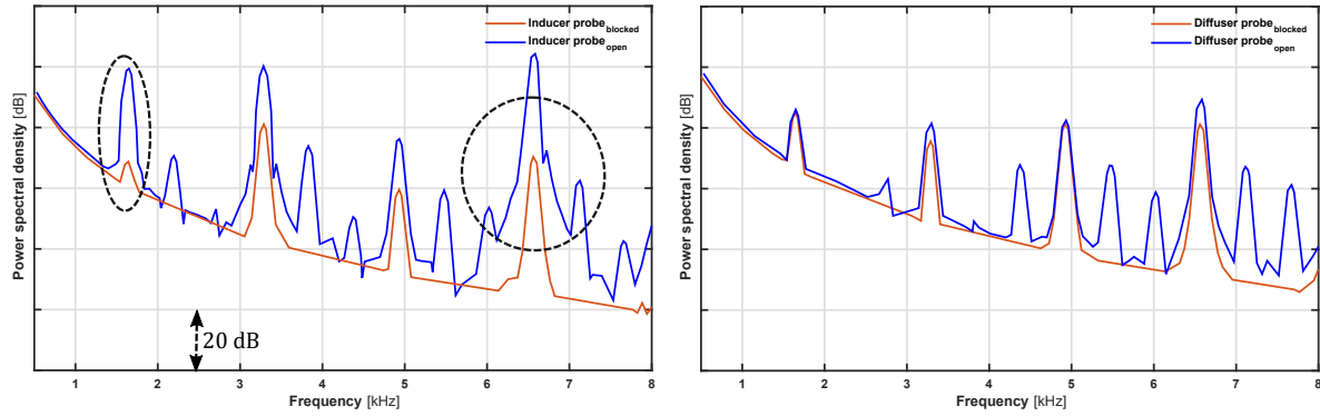
Figure 14: Experimental (top) and numerical (bottom) spectra of inducer (left) and diffuser (right) probe for open (blue) and blocked (orange) compressor configurations operating at design conditions.
