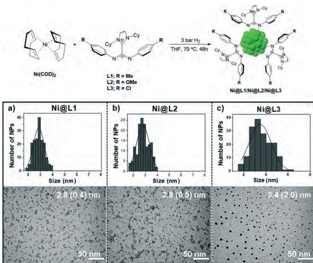
Fig. 1 Top: Synthesis of the nickel nanoparticles stabilized by \text{ICy}^{-(\text{Ar})}\text{NCN} (Ni@L1, Ni@L2 and Ni@L3). Bottom: TEM images and size distribution histograms of (a) Ni@L1, (b) Ni@L2 and (c) Ni@L3.
