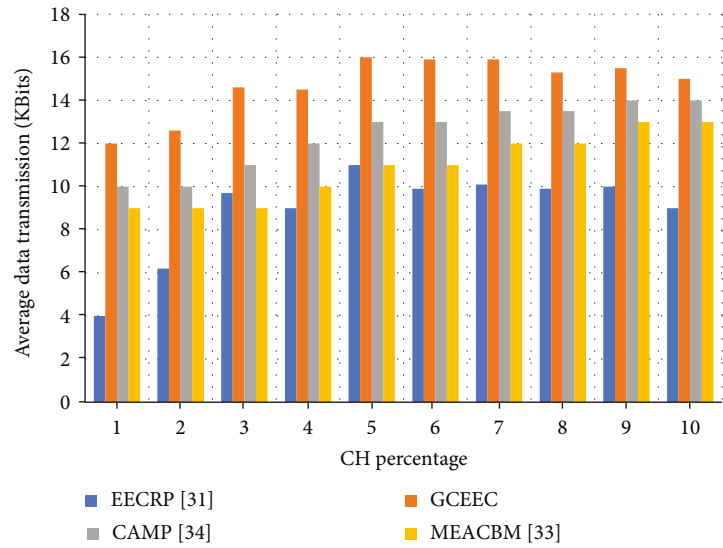
FIGURE 12: Average data transmission with different numbers of CHs.
