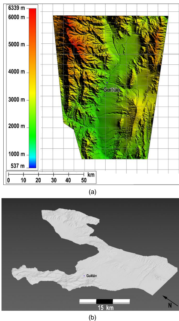
Figure 3: Guitián's surrounding topography: a) SRTM image; and b) cropped perspective view of the TIN.
