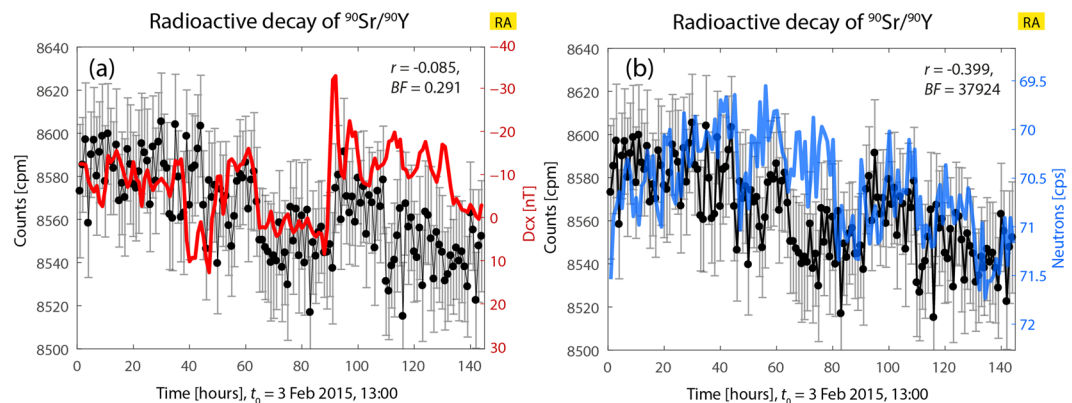
Figure 6. Decay rate of ^{90}\text{Sr}/^{90}\text{Y} vs. Dcx and neutron counts; (a) uncertain good correlation between both variables due to the high transient, (b) Good correlation exists in (b). In (a) and (b): decay rates oscillations are >4 cpm. In (a) and (b): decay data oscillations are >7 cpm.
