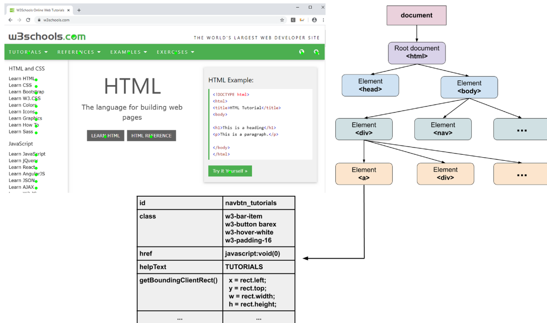
Figure 3. The state of a graphical user interface can be described as a widget tree.
