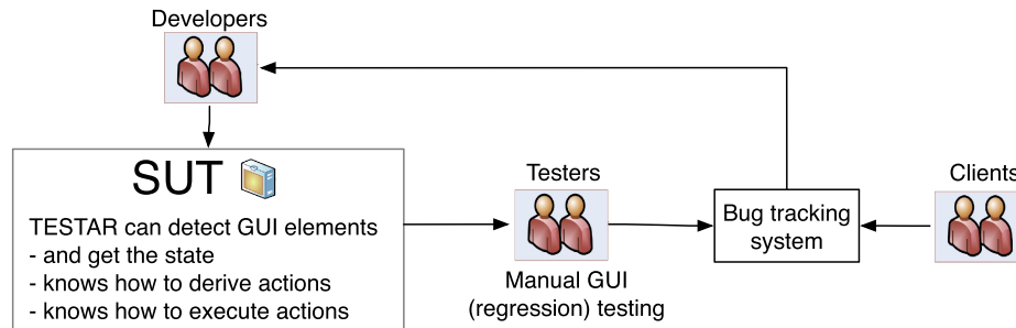
Figure 13. Similar components and interactions of the cases for generalization through architectural analogy. GUI, graphical user interface; SUT, system under test.
