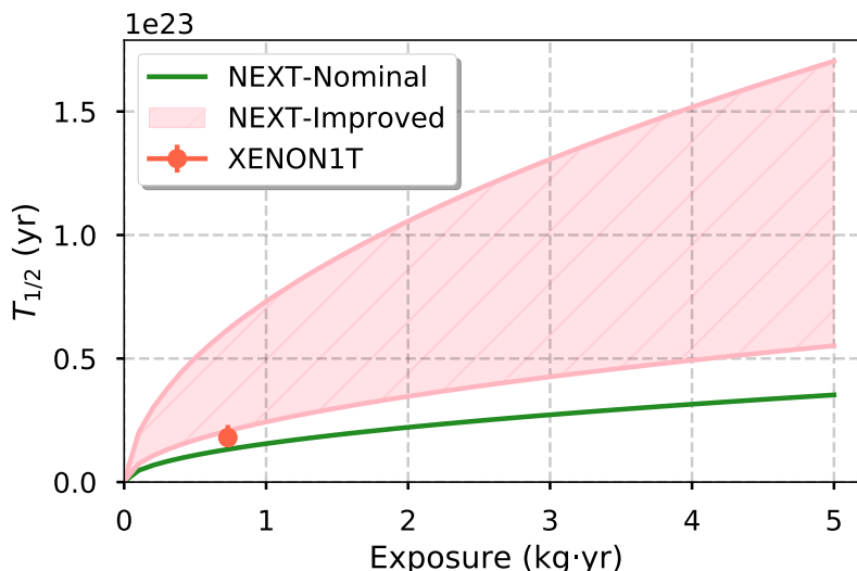
Figure 11. NEXT nominal (green curve) and improved (red band) half-life sensitivity to ^{124}\text{Xe} 2\nu ECEC versus exposure, compared with the XENON1T measurement in reference [10] (red marker).
