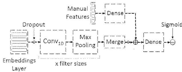
Figure 6. Architecture of ConspiDetector.
