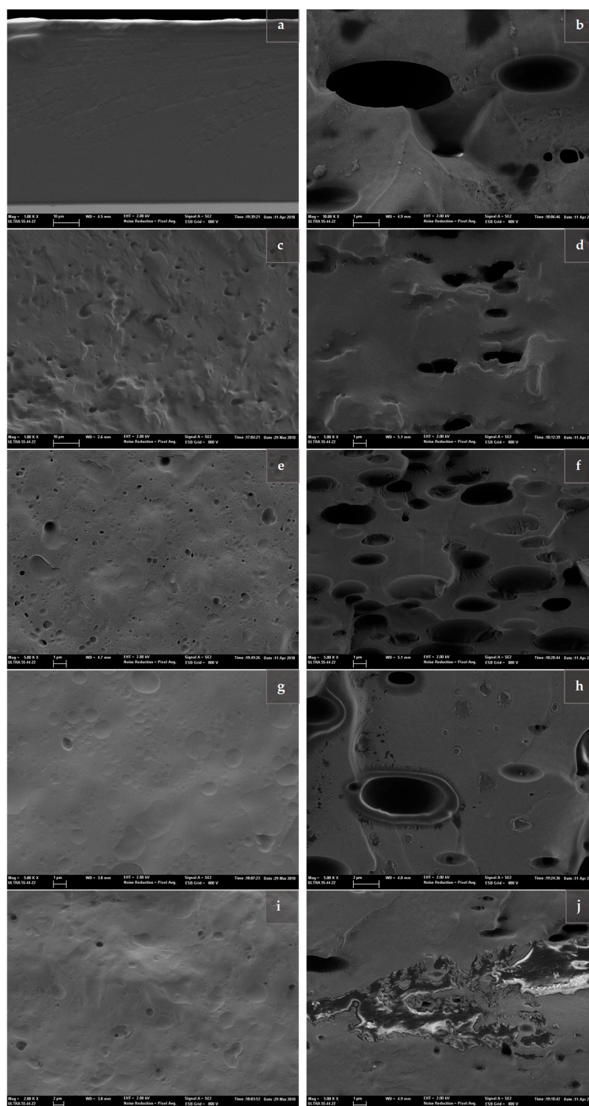
Figure 3. FESEM micrographs of the cross-section of F-PVA and P-PVA films with CA-loaded liposomes (CA: LEC: 1:1) using different types of lecithin (soy lecithin enriched in phosphatidylcholine PC (SL-PC), soy lecithin (SL) and sunflower lecithin (SFL)) and the sonication method. (a) P-PVA with free CA; (b) F-PVA with free CA; (c) P-PVA with CA-free SL-PC; (d) F-PVA with CA-free SL-PC; (e) P-PVA with CA-loaded SL-PC; (f) F-PVA with CA-loaded SL-PC; (g) P-PVA with CA-loaded SL; (h) F-PVA with CA-loaded SL; (i) P-PVA with CA-loaded SFL; (j) F-PVA with CA-loaded SFL.
