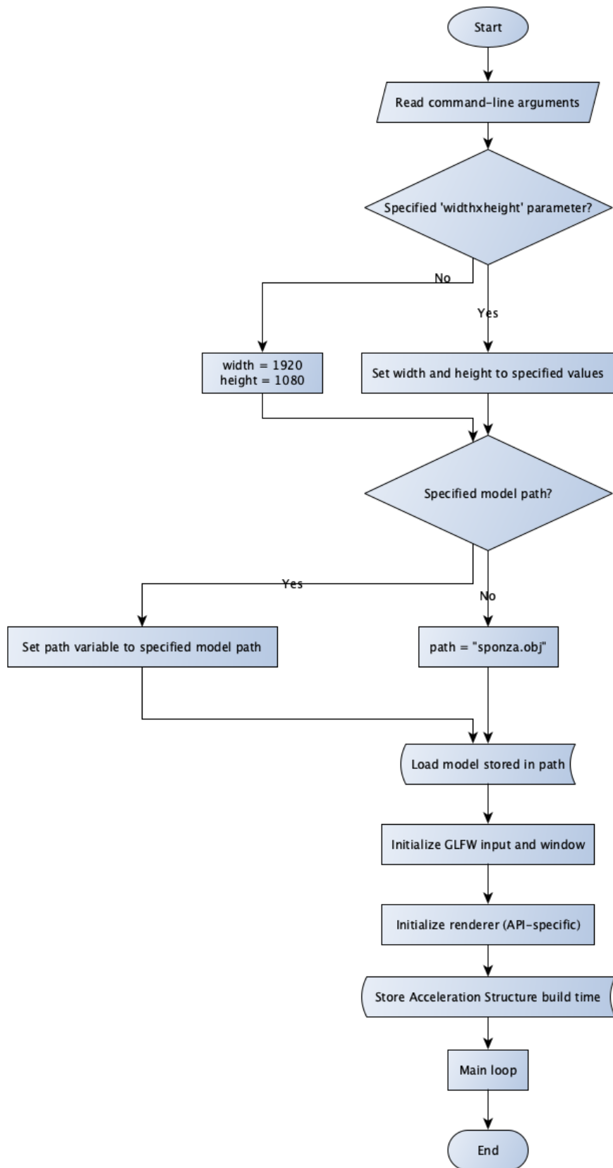
Figura 4.3: Renderer initialization process flow chart.
