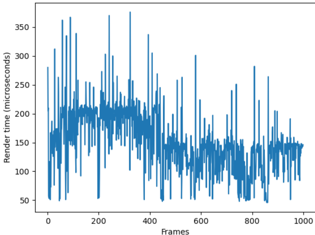
Figura 6.9: Time taken for rendering 1000 frames when drawing the BMW 3D model at 1280x720, using ray tracing. We have removed the first frame time since it took too long to draw in comparison with the rest.
