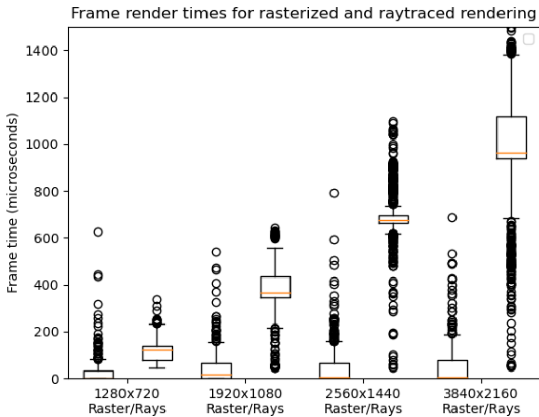
Figura 6.2: Single frame rendering time when drawing the Viking Room 3D model at a range of reasonable resolution, using ray traced and traditionally rasterized graphics. As with the memory consumption graph, we see how the two of them take longer to finish in higher resolutions, while the rasterized renderer greatly outperforms the ray traced one.
