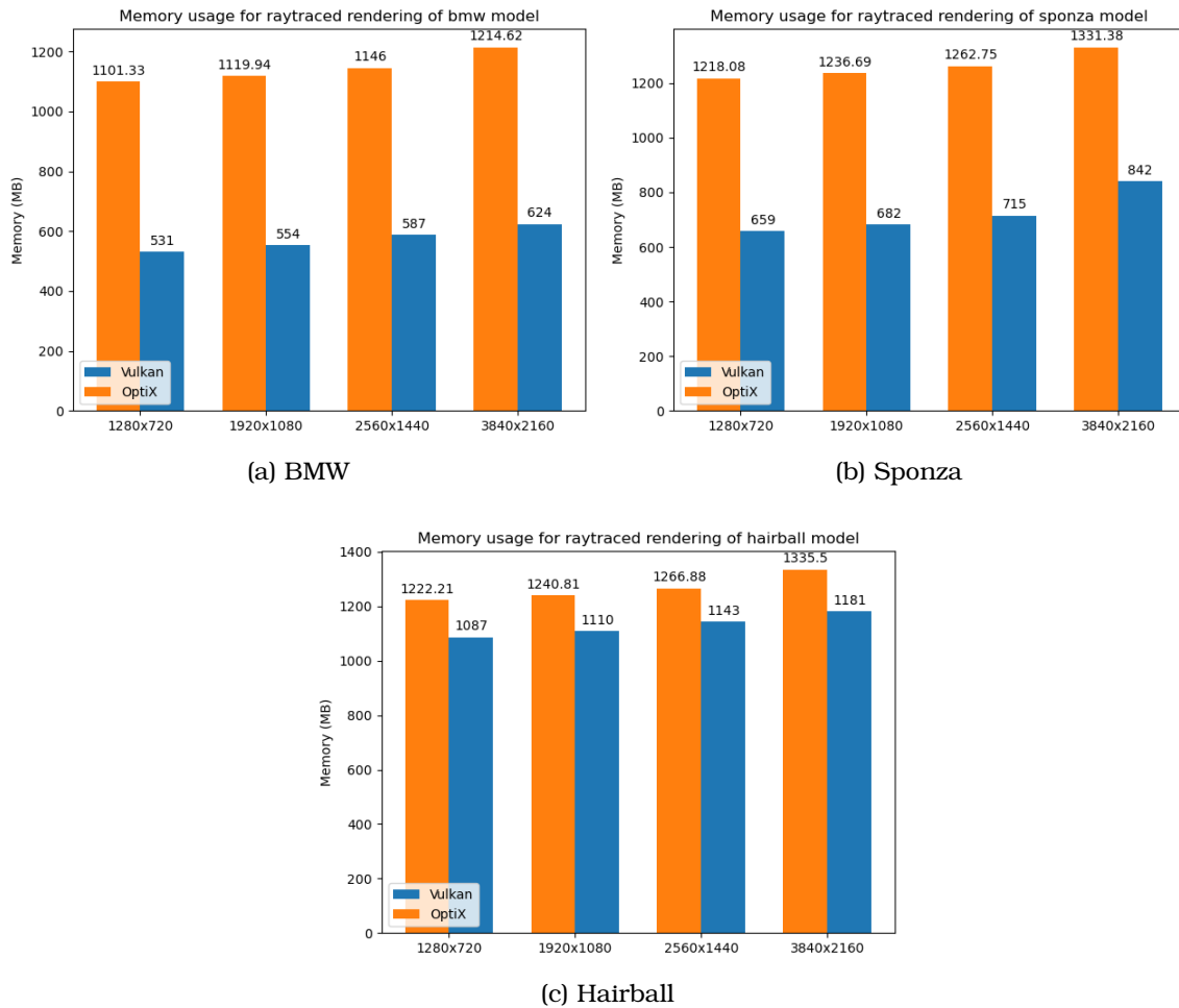
Figure 6.3: Memory consumption of OptiX and Vulkan (raytraced) when rendering the 3D models BMW, Sponza and Hairball.
