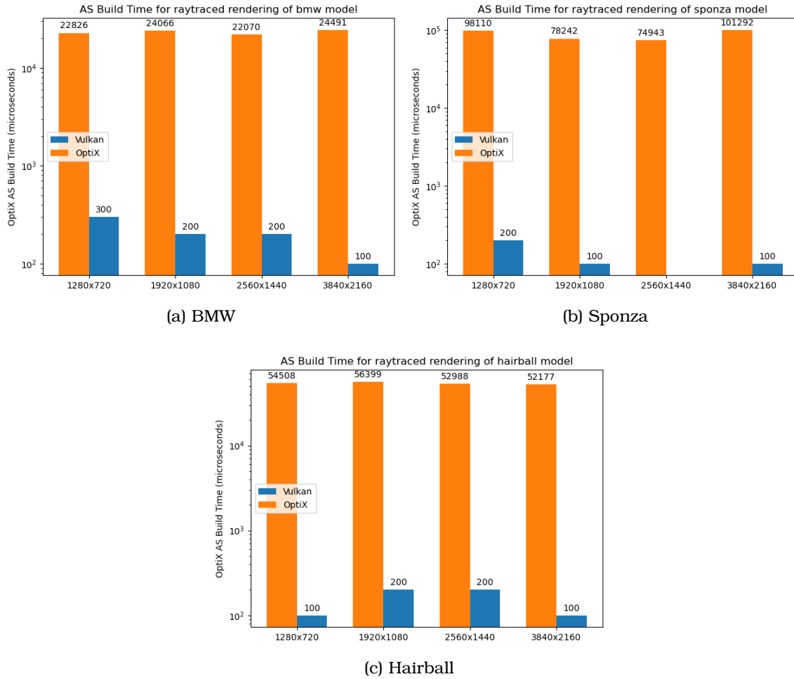
Figure 6.4: Acceleration Structure Build Time of OptiX and Vulkan (raytraced) when rendering the 3D models BMW, Sponza and Hairball. Sorted by rendering resolution.
