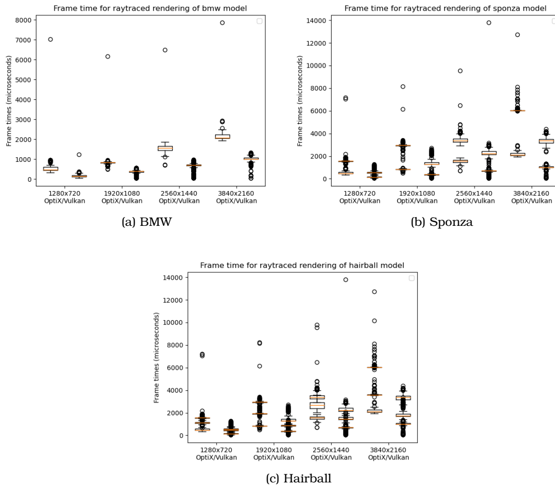
Figure 6.10: Frame rendering times for each 3D model (BMW, Hairball and Sponza) across both libraries and 4 reasonable resolutions, from 720p to 4k.
