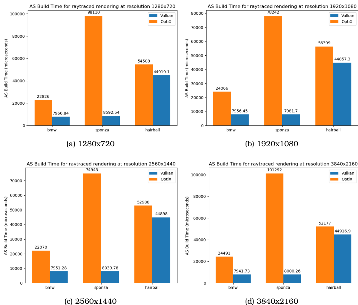
Figura 6.5: Acceleration Structure Build Time of OptiX and Vulkan (raytraced) when rendering the 3D models BMW, Sponza and Hairball. Sorted by model.
