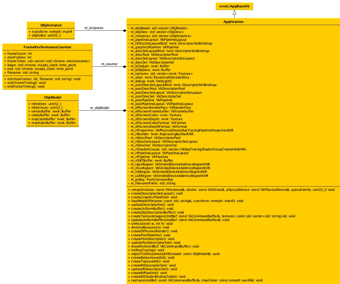
Figura 4.1: UML class diagram for the raytraced Vulkan renderer.
