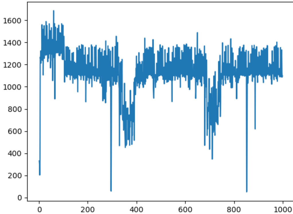
Figura 3.1: Render times over 1000 frames with a frame buffer resolution of 7680x4320, while drawing the model of a viking room with textures. It can be observed how in a very short span of time, the rendering time of the exact same geometry and effects can hugely change.
