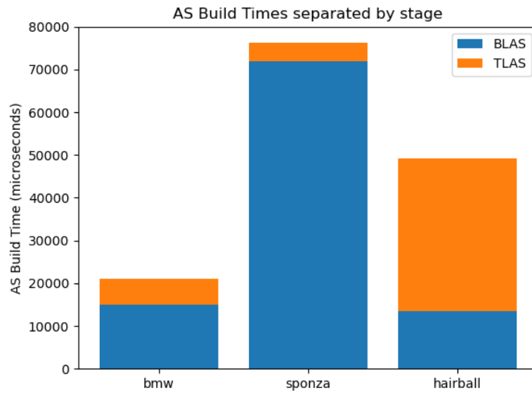
Figura 6.6: Acceleration Structure Build Times for each model, divided between the TLAS and BLAS phases. We see great discrepancies in the distribution of time in each case.
