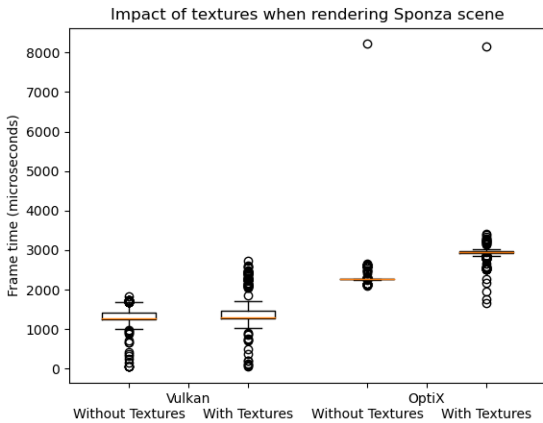
Figura 6.11: Sponza scene rendered in Vulkan and OptiX, both with and without textures, to compare how these affect render times.
