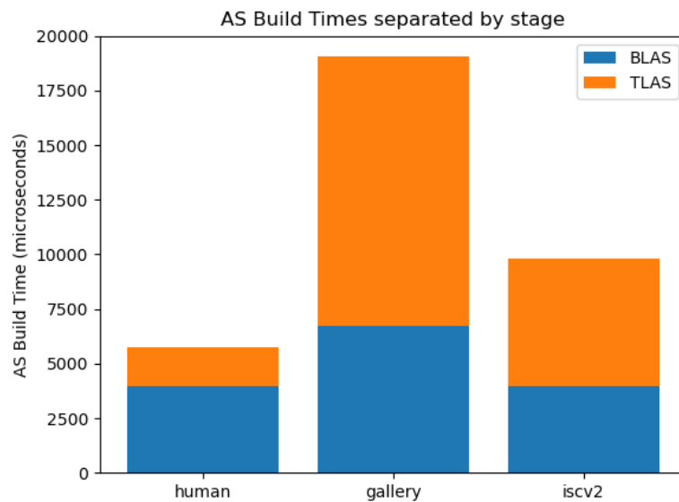
Figura 6.7: Acceleration Structure Build Times divided between the TLAS and BLAS phases for the extra set of models (Human, ISCV2 and Gallery).
