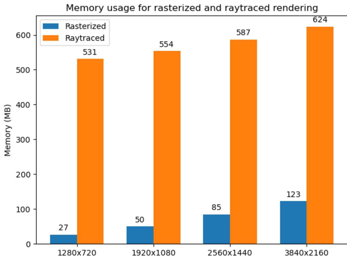
Figura 6.1: GPU memory consumption when rendering the Viking Room 3D model at a range of reasonable resolutions, using ray traced and traditionally rasterized graphics. We can see a significant difference between the two, as well as an expected increase as resolutions get higher.
