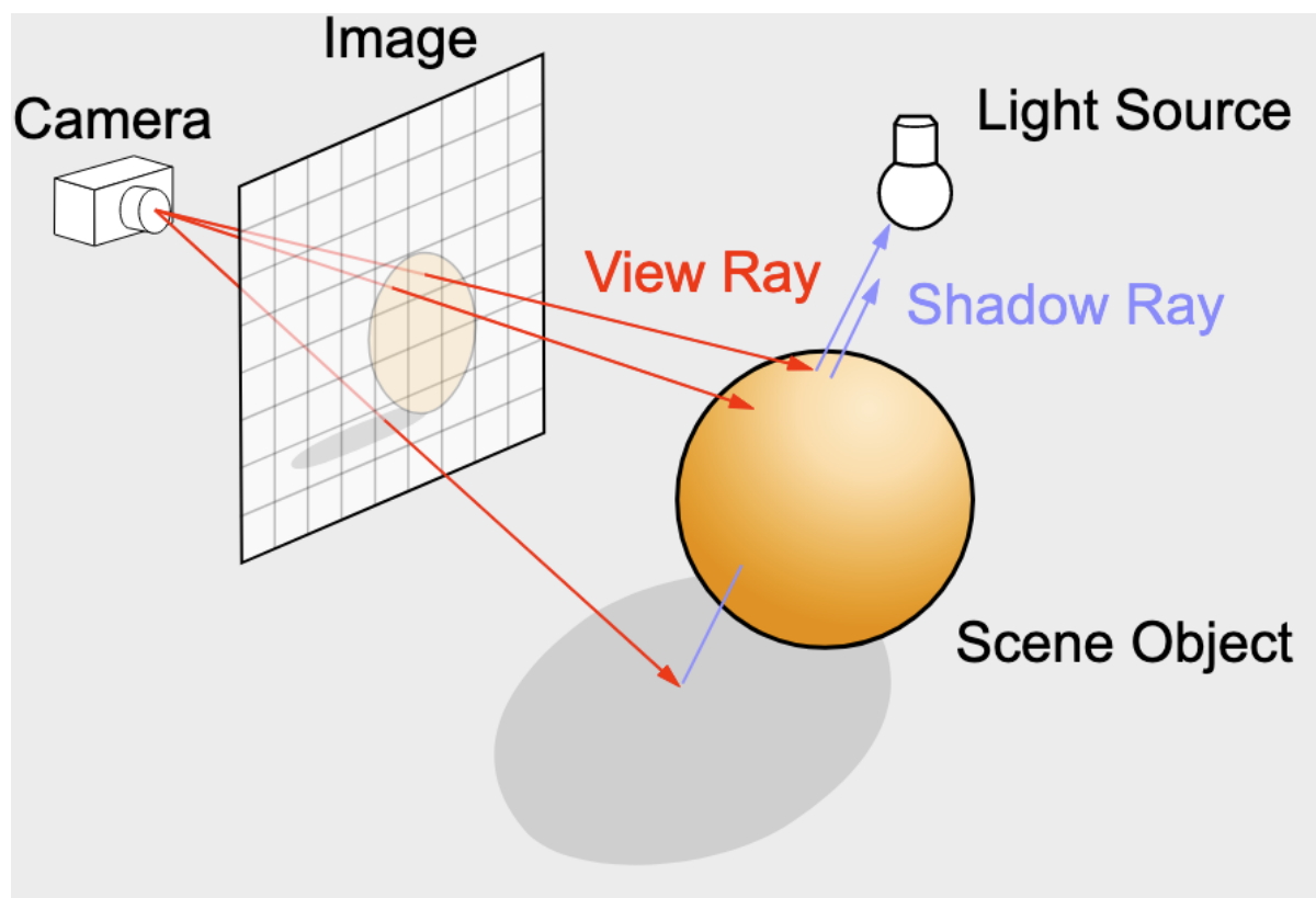
Figura 2.2: Overview of the ray tracing algorithm with spheres as our only geometry and a single light source.
