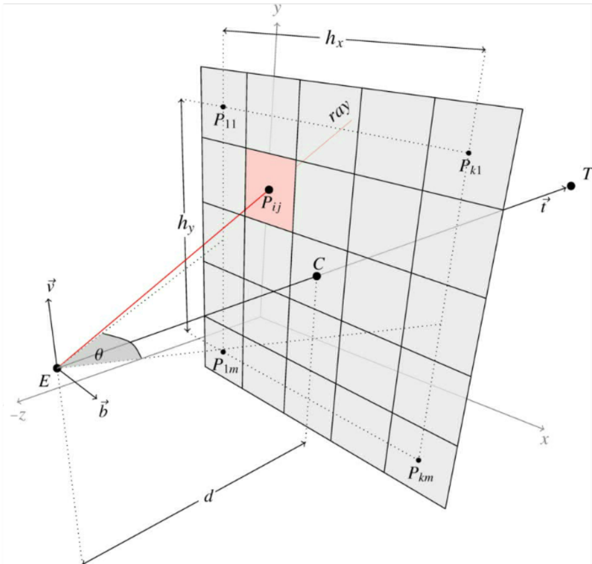
Figura 2.3: Ray tracing schema with all the input components.
