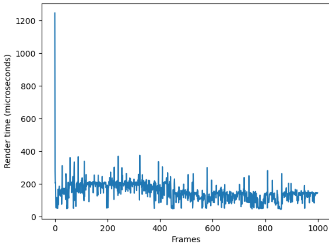
Figura 6.8: Time taken for rendering 1000 frames when drawing the BMW 3D model at 1280x720, using ray tracing. We see how the first frame takes much longer than the rest of them to draw.
