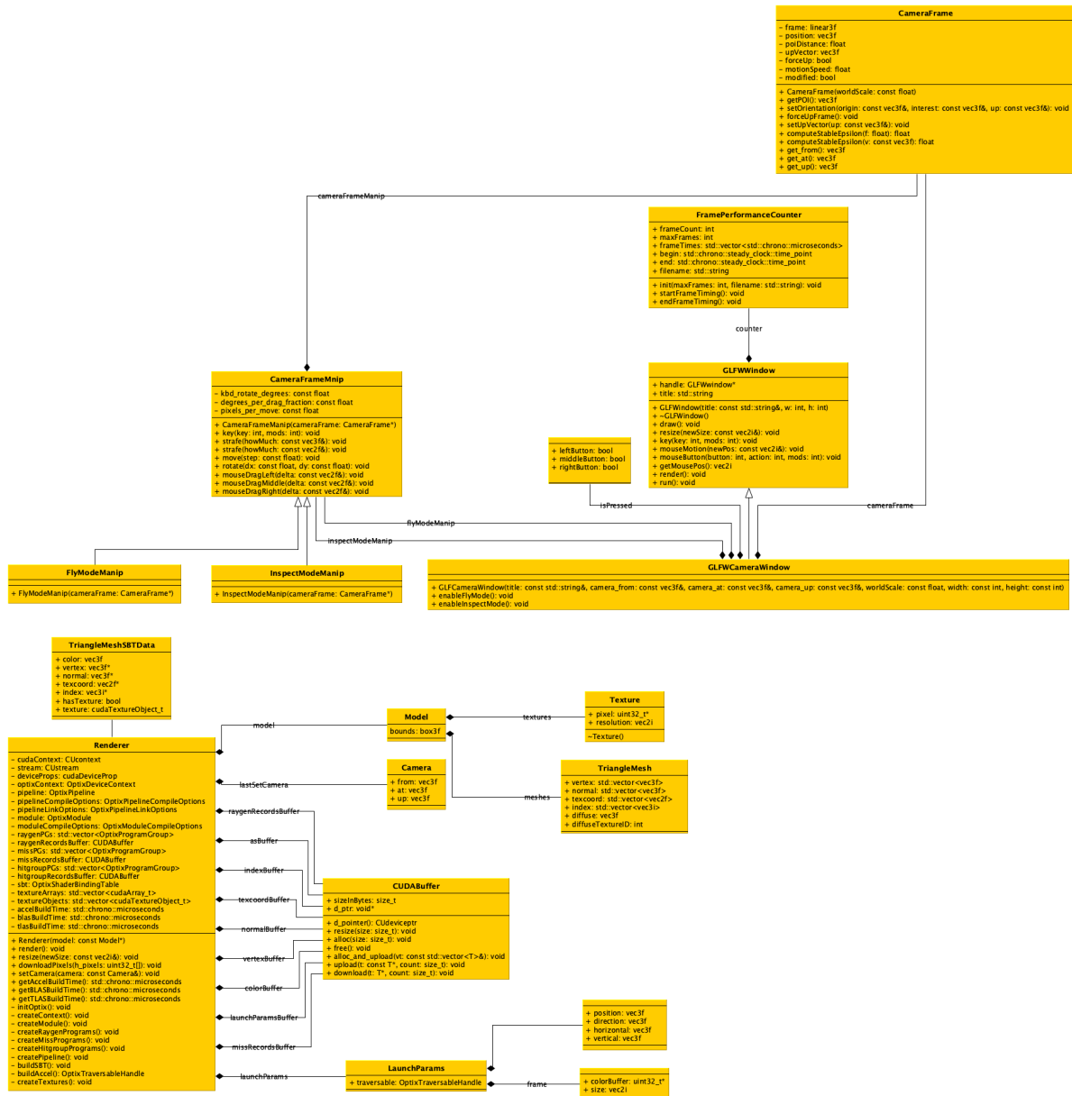
Figura 4.2: UML class diagram for the OptiX ray tracer.
