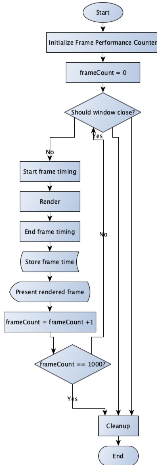
Figura 4.4: Renderer main loop flow chart.
