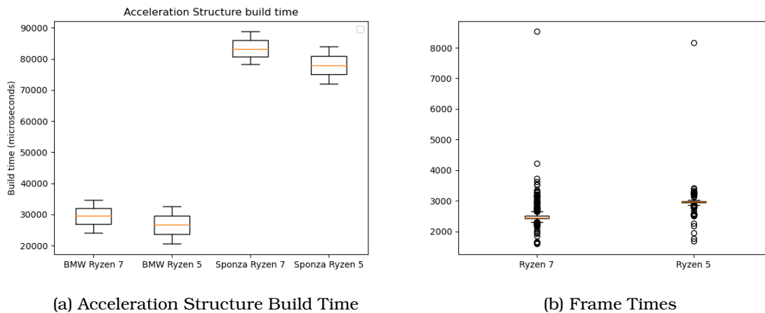
Figura 6.12: Acceleration Structure Build Time and Frame Render Time comparison in OptiX when using an Nvidia 2070 Super in two systems with different CPUs. We see how a faster CPU means better performance in both cases.
