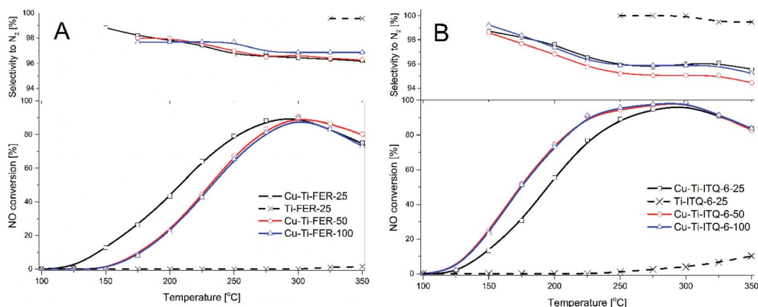
Fig. 9 Results of NH 3 -SCR catalytic tests for copper modified Ti-FER (A) and Ti-ITQ-6 (B) catalysts.
