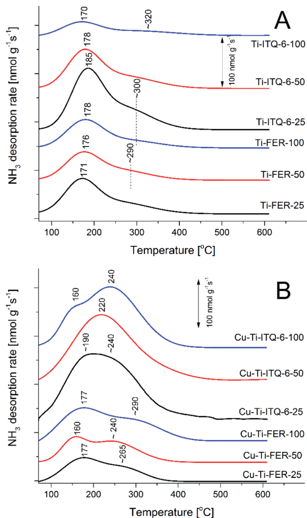
Fig. 8 NH 3 -TPD profiles of obtained for Ti-FER and Ti-ITQ-6 zeolites (A) and their copper modified forms (B).
