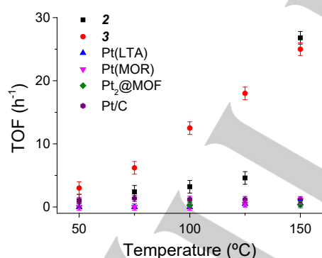
Figure 4. Temperature–programmed WGS catalyzed by 3 and other Pt–supported catalysts in–flow.
