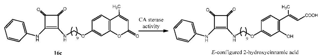
Scheme 4. Mode of inhibition of squaramide 16c .
