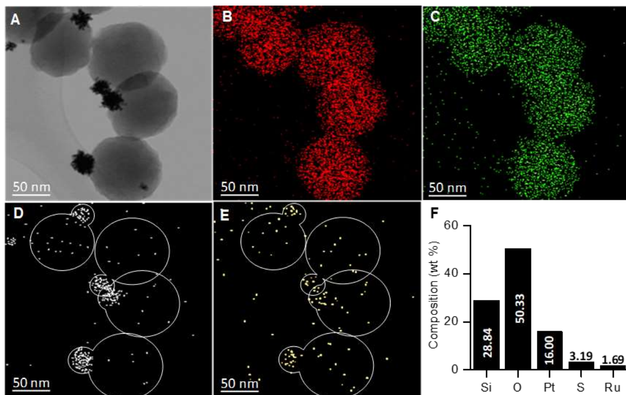
Figure 2. STEM image (A), STEM-EDX elemental mapping of Si atoms (B), O atoms (C), Pt atoms (D), S atoms (E) and wt % composition detected (F) in S 1 Janus Pt-MSNPs.
