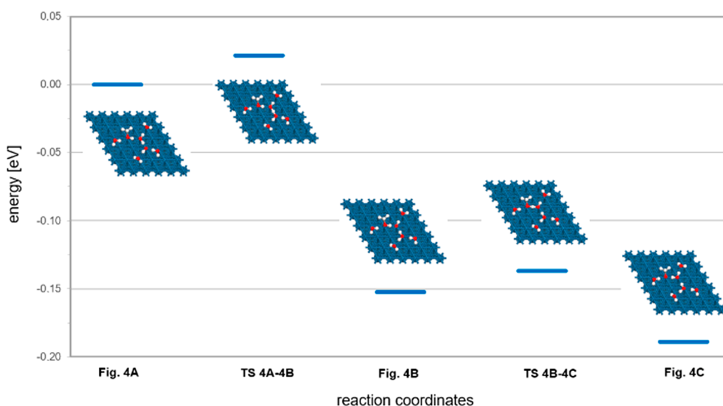
Figure 5. Energy profiles for the virtually barrier-less methanol activation on the Pt(111) surface in the presence of adsorbed OH (using the adsorption configurations from Figure 4A–C and the corresponding transition states).
