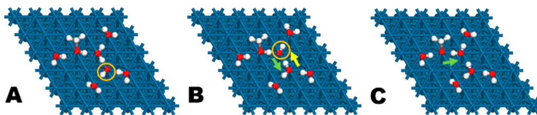
Figure 4. Adsorption configurations on the Pt(111) surface in water involving methanol, adsorbed OH, and their recombination to yield water. (A) Adsorbed methanol in the presence of nonadjacent adsorbed OH. (B) Coadsorbed OH and methanol on adjacent locations. (C) Adsorbed methoxy formed with the aid of adsorbed OH to yield water. Orange circles highlight adsorbed OH locations and yellow and green arrows emphasize adsorbed OH and hydrogen evolutions with respect to the previous state, respectively.
