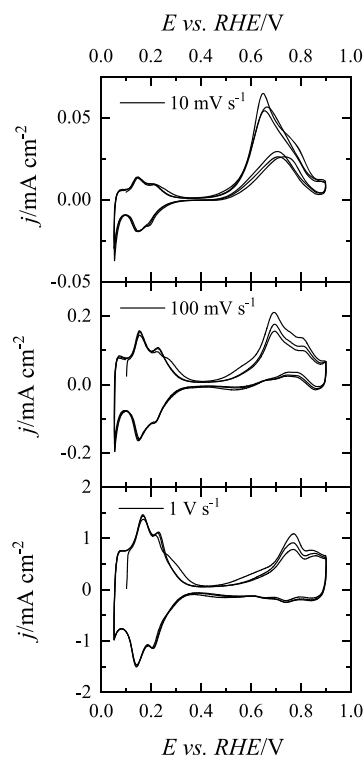
Figure 3. Voltammetric profiles (three full cycles) for the Pt(110) electrode in 0.1 M HClO 4 + 0.1 mM MeOH at selected scan rates.
