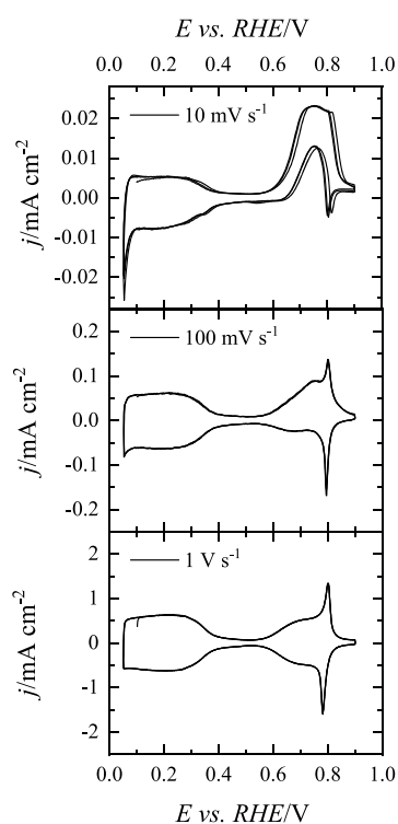
Figure 1. Voltammetric profiles (three full cycles) for the Pt(111) electrode in 0.1 M HClO 4 + 0.1 mM MeOH at selected scan rates.
