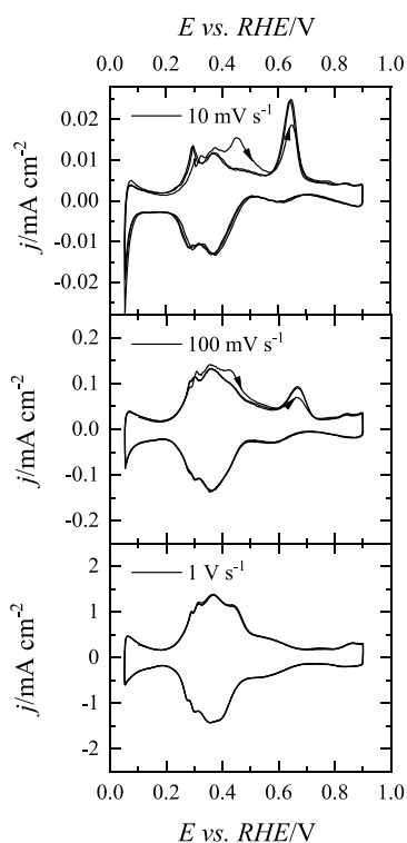
Figure 2. Voltammetric profiles (three full cycles) for the Pt(100) electrode in 0.1 M HClO 4 + 0.1 mM MeOH at selected scan rates. The arrows mark the first positive scan direction of the profile.
