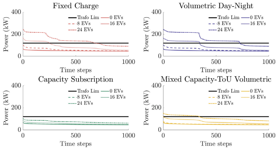
Fig. 9. The 1000 highest load time-steps of the load duration curve for selected EV numbers and transformer size of 120 kW.
