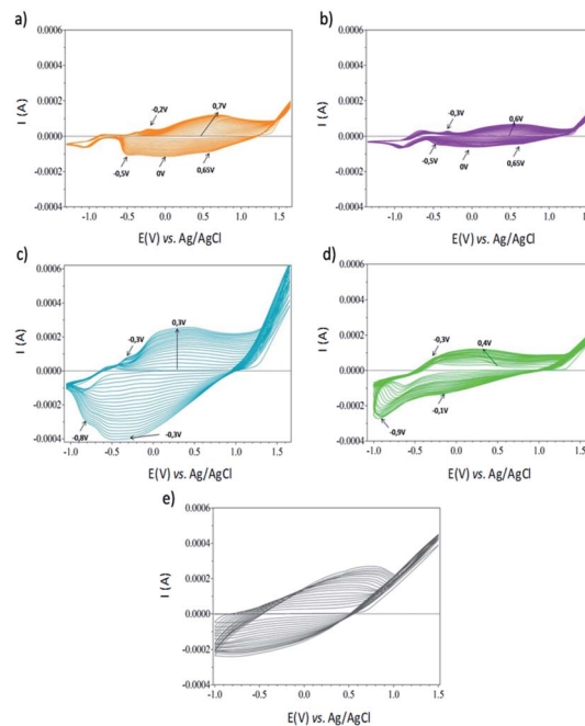
Fig. 1 Cyclic voltammograms for the electropolymerization of 10 mM EDOT and 10 mM (a) Cs[1]-Cl 2 ; (b) Cs[1]-Cl 4 ; (c) Cs[1]-Cl 6 ; (d) Cs[1]-I 6 ; and (e) PSS.
