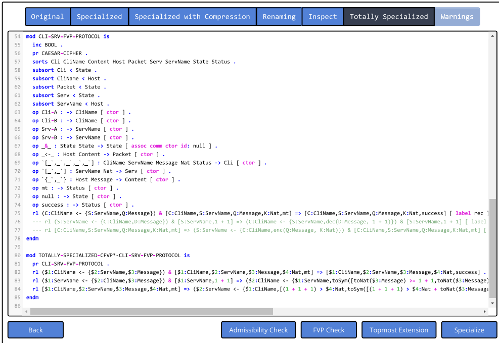
Fig. 16. Total evaluation of the Client-Server Communication Protocol with FVP.
