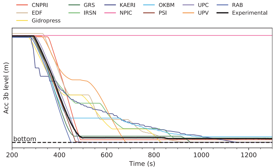
Fig. 16. Accumulator 3 level.
