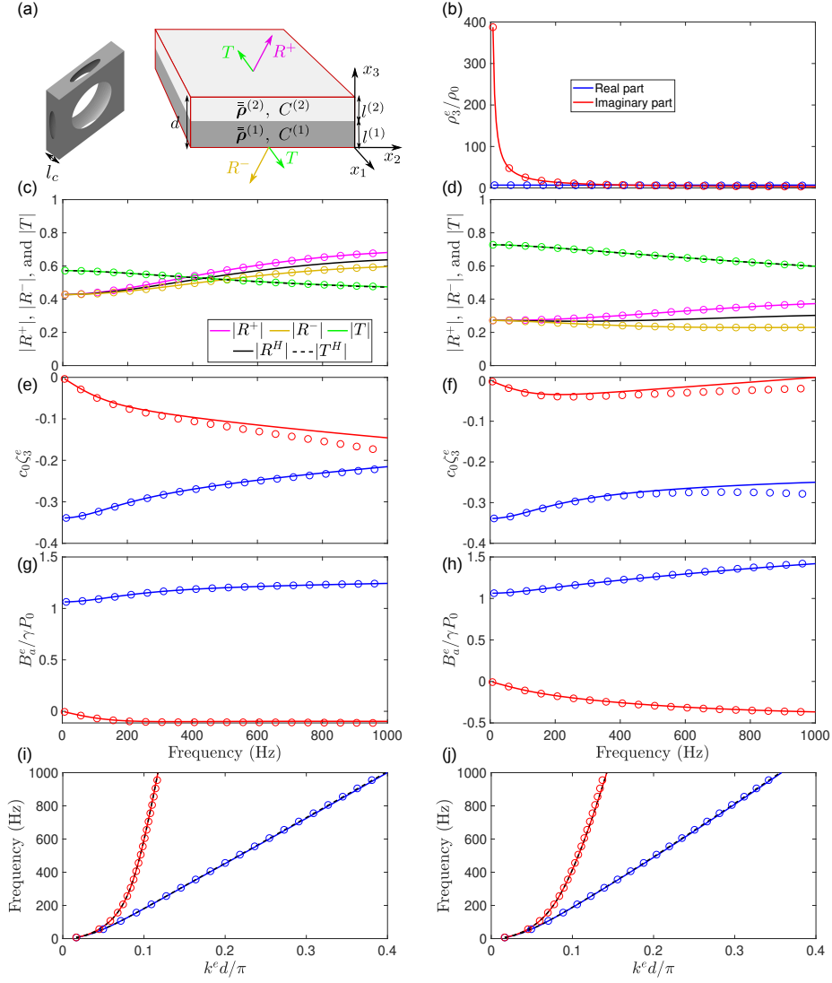
Figure 2: [Color online] Sketch of the laminate unit cell together with the micro-structure unit cell (a). Absolute value of the reflection and transmission coefficients (c-d) of a L = d -thick laminate ( N = 1 ), normalized Willis coupling (e-f), normalized apparent bulk modulus (g-h), and dispersion relation -black lines depict the classical homogenization results- (i,j) for (0, 0) and (\frac{\pi}{3}, \frac{\pi}{6}) . The normalized density along the \mathbf{x}_3 -direction is depicted in (b). Real (blue curves) and imaginary (red curves) parts of each element are depicted. Elements calculated with the effective parameters are plotted in solid line and those numerically evaluated are plotted with circle symbols.
