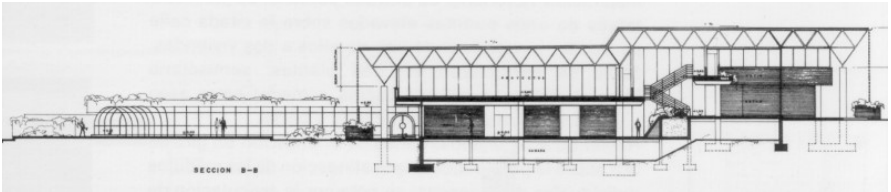
Figure 5. Section of the School of Architecture at Universidad de Navarra
