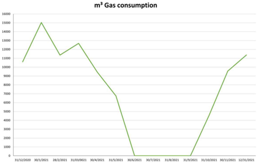
Figure 8. Gas consumption during 2021 at School of Architecture. Monthly gas consumption during 2021
