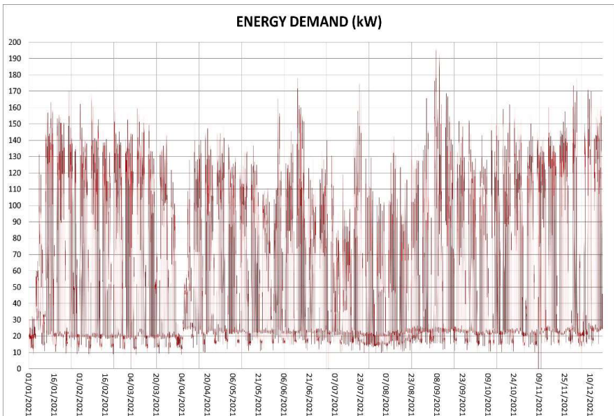
Figure 7. Electrical consumption during 2021 at School of Architecture. Hourly energy consumption during 2021
