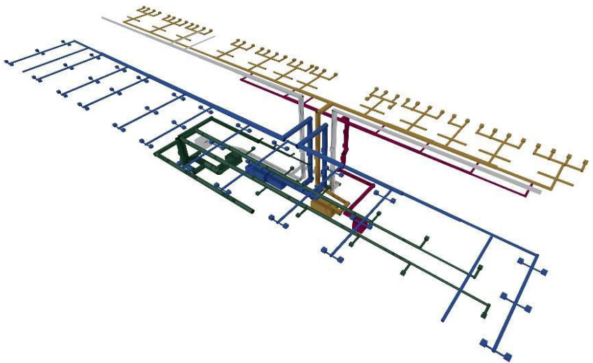
Figure 9. HVAC duct distribution at the School of Architecture. Orange offices, blue workshop, pink classroom and green laboratory
