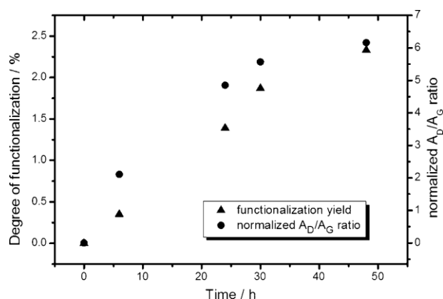
Figure 1. Comparison of the degree of functionalization (determined by TGA) with the normalized A_D/A_G ratio (from Raman spectra) for the reaction of SWCNTs with (PhS)_2 as a function of the reaction time.
