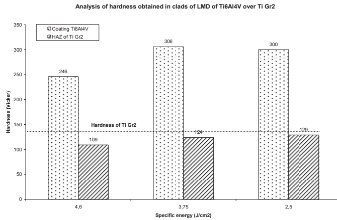
Figure 5. Analysis of hardness of clads number 17, 9 and 14 with process parameters of Table 7.
