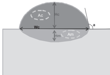
Figure 2. Dimensional analysis of single clads. Parameters measured. Wc: width of clad, Hc: height of clad, Hm: deep of dilution of clad material on substrate material, Ac: area of clad, Am: area of dilution, a: angle of clad.
