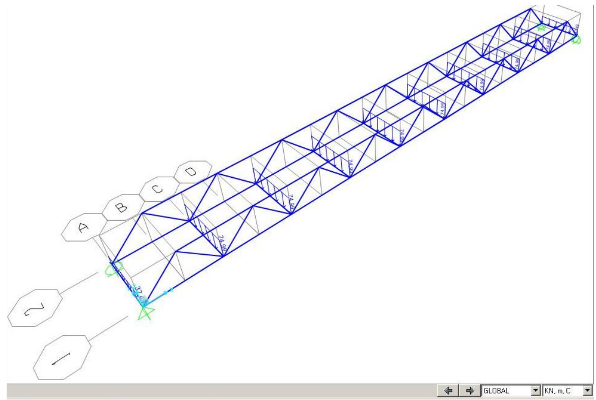
Figura 6: Agua (24,997 kN/m)
