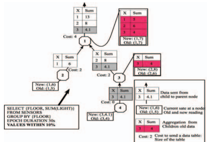
Fig.5. In-network aggregation query using TiNA [53].
