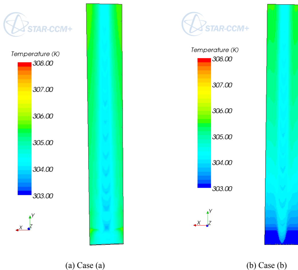
Figure 9. External building face temperature comparison
