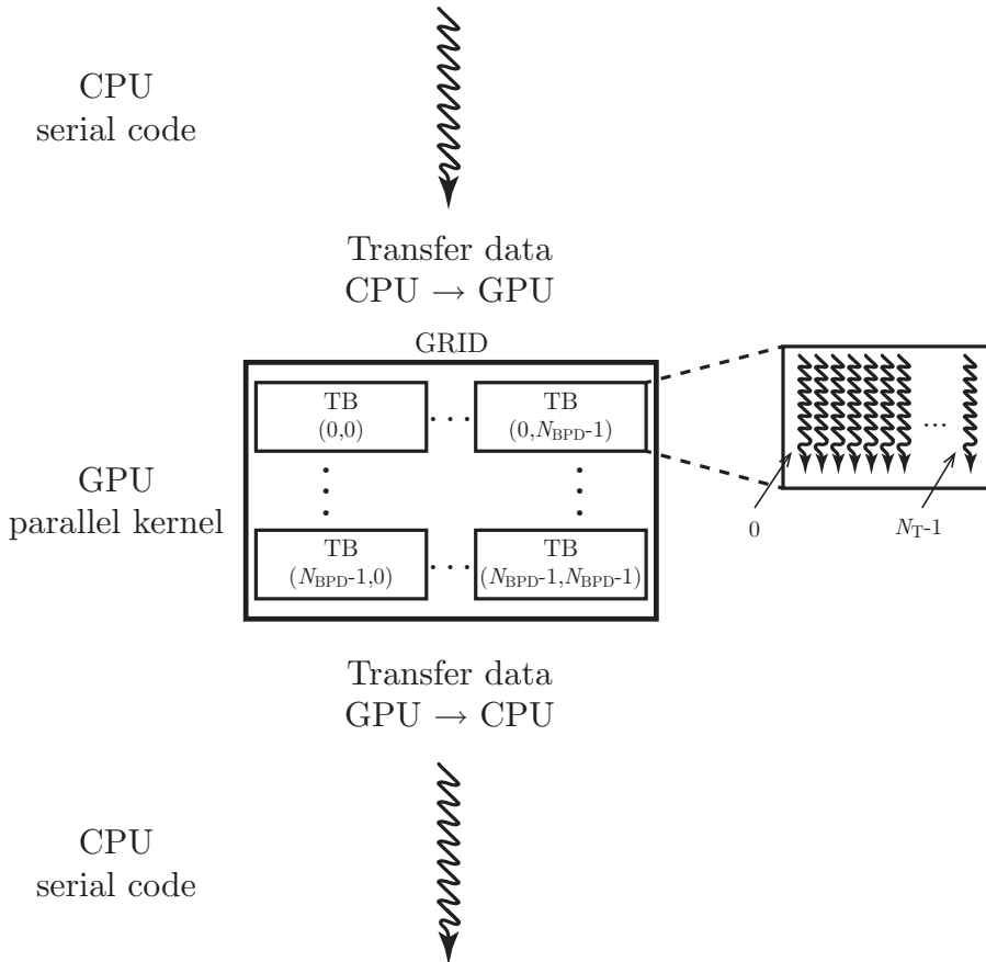
Figure 5.1: Example of execution of a CUDA program using a 2-dimensional grid with N_{\text{BPD}} blocks per dimension and 1-dimensional block with N_{\text{T}} threads.
