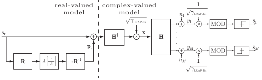
Figure 3.5: LRAP-linear scheme.
