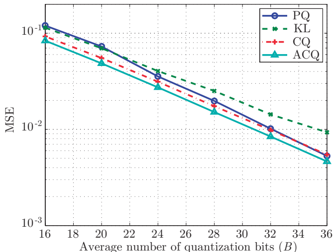
Figure 7.18: MSE for N_t = 4 , d = \lambda and different average number of quantization bits.
