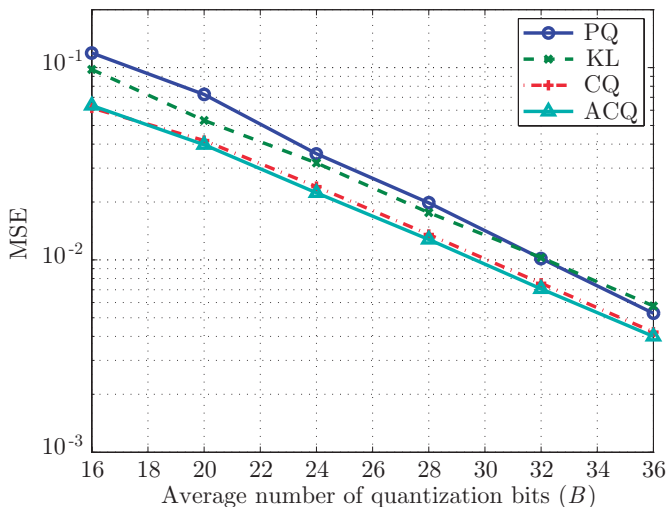
Figure 7.17: MSE for N_t = 4 , d = \lambda/2 and different average number of quantization bits.
