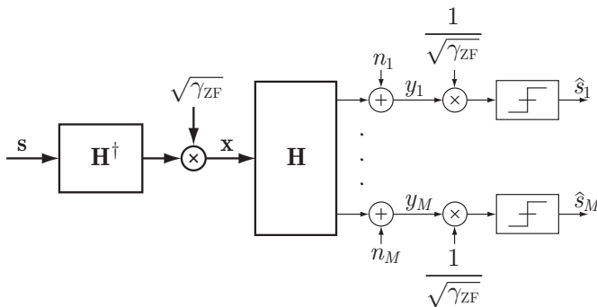
Figure 3.2: ZF precoding scheme.
