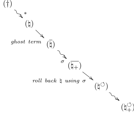
Figure 2: States obtained using the super-lazy intruder optimization
