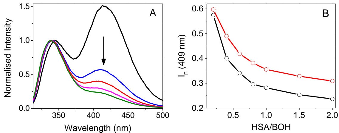
Figure 1. (A) Fluorescence spectra (normalised at the short-wavelength maximum) of ( S )-BOH in PBS ( \lambda_{\text{exc}} = 308 \text{ nm} , air, 10^{-4} \text{ M} ) after addition of increasing amounts of HSA. The ( S )-BOH/HSA molar ratios are 1:0 (black), 1:0.2 (blue), 1:0.4 (red), 1:0.8 (magenta), and 1:2 (green). (B) Plot of the fluorescence intensity at 409 nm vs HSA/BOH molar ratio for ( S )-BOH (black) and ( R )-BOH (red). Adapted with permission from J. Phys. Chem. B , 2012, 116 , 14839-14843. Copyright 2012 American Chemical Society.
