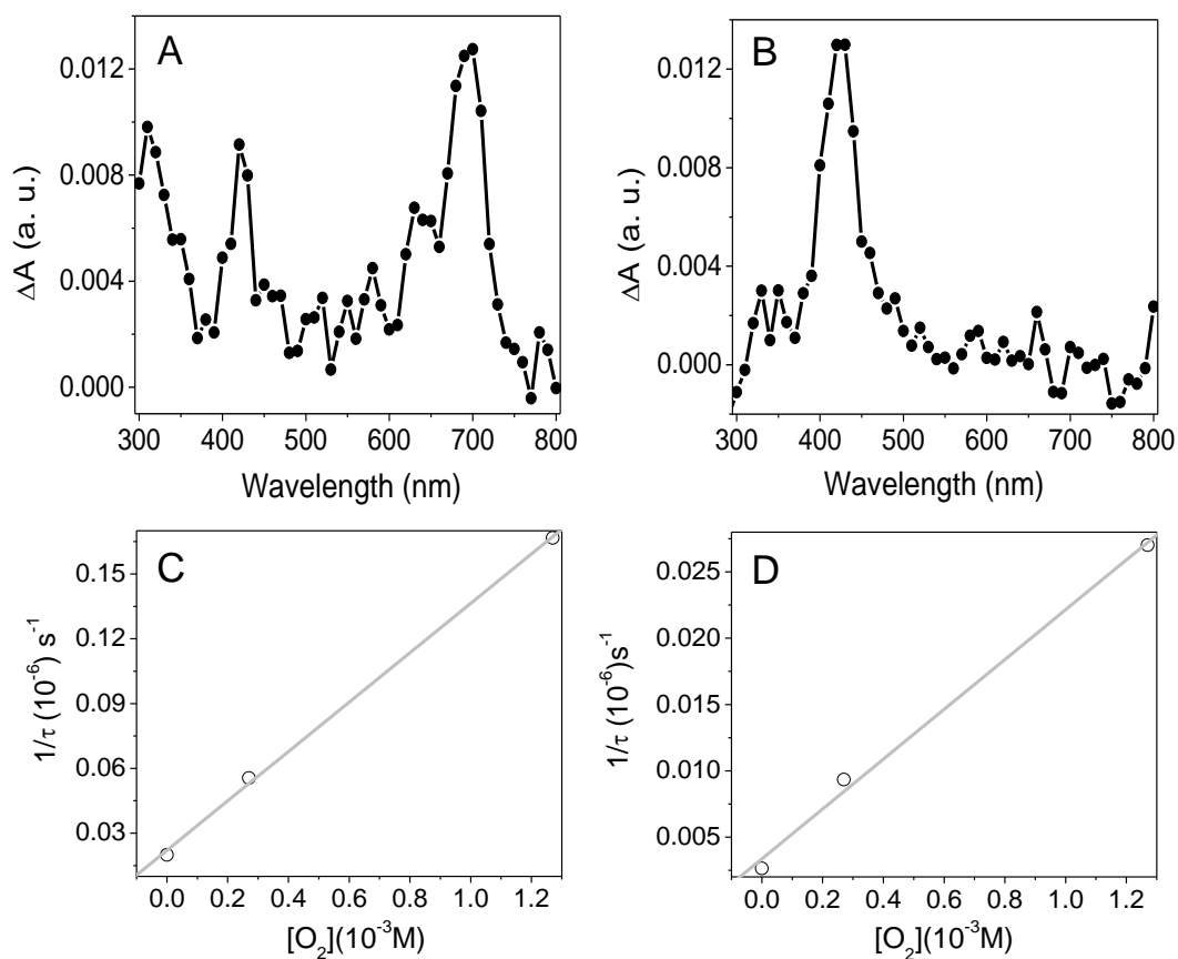
Figure 14. Laser flash photolysis in PBS, under air at \lambda_{\text{exc}} = 355 \text{ nm} . Transient absorption spectra of (S) -ANP in the absence (A) and in the presence of HSA, at 1:1 molar ratio (B), recorded 1 \mu\text{s} and 2.9 \mu\text{s} after laser pulse, respectively. Stern-Volmer plots for quenching of the (S) -ANP triplet state by oxygen in site I (C) or in site II (D) of HSA. Adapted with permission from Org. Lett. , 2011, 13 , 3860-3863. Copyright 2011 American Chemical Society.
