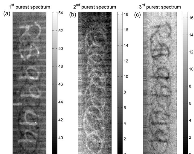
Figure 5. Distribution maps for the first three purest pixel estimations of MCR-ALS.
