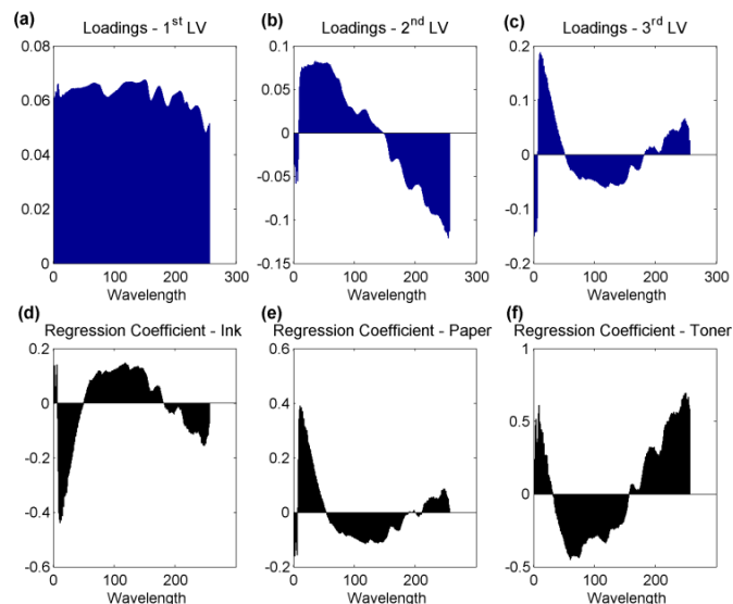
Figure 8. Sample 1.1: Loading plots from the PLS-DA model for the first three latent variables (a), (b) and (c); Regression coefficient plots of PLS-DA model for (d) ink, (e) paper and (f) toner.
