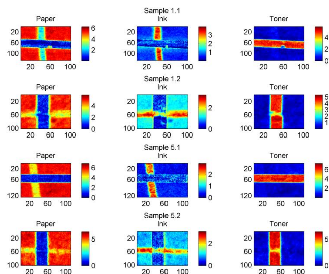
Figure 10. Distribution maps for two different pairs of samples. The 1 st , 2 nd and 3 rd columns show the paper, ink and toner distribution maps, respectively, for samples 1.1 (first row), 1.2 (second row), 5.1 (third row) and 5.2 (fourth row). In samples 1.1 and 5.1 the ink line lies over the toner line; in samples 1.2 and 5.2 the ink line lies below the toner.
