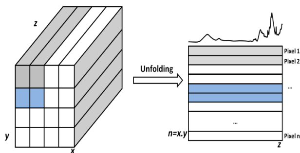
Figure 1. NIR image as a three-dimensional array (hyperspectral cube) and the unfolding process to give to a two-dimensional matrix.
