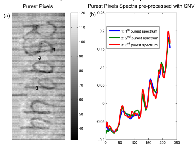
Figure 4. (a) purest pixels location; (b) purest pixels spectra pre-processed with SNV and used as initial estimates in MCR-ALS.
