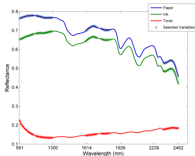
Figure 9. PLS-DA selected variables (scatter dots) from paper (blue line), ink (green line) and toner (red line).
